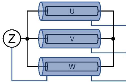
Fig. 15. Configuration topology for impedance measurement of the cables
