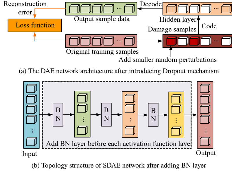
Fig. 5. The two optimization methods of SDAE
