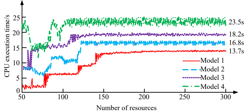
Fig. 10. CPU consumption of different models in the diagnosis process
