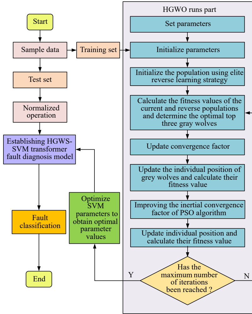
Fig. 4. Flowchart of HGWO-SVM
