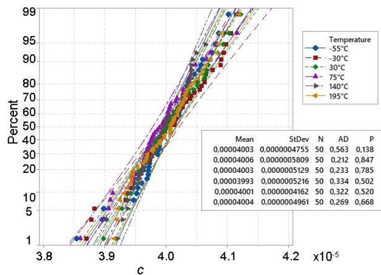
Fig. 14. Probability plot, the distributions of parameter c in temperature range of -55 to 195^\circ\text{C}
