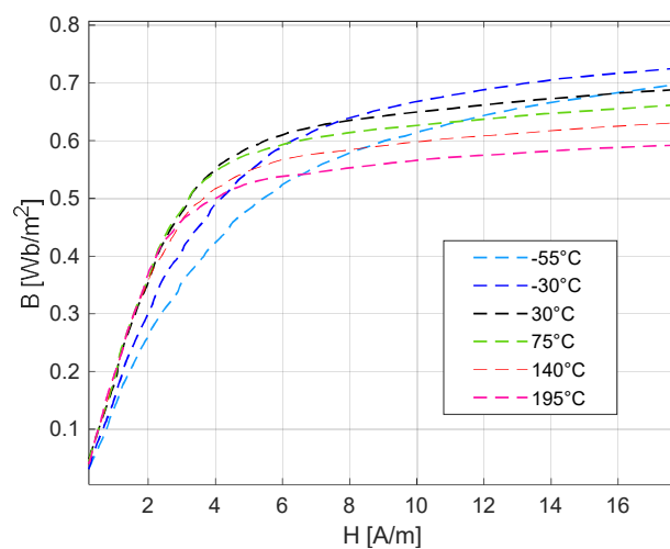
Fig. 17. Anhysteretic magnetisation curves of the ASTM A753 Alloy 4, measured in the temperature range of -55 to 195^{\circ}\text{C}
