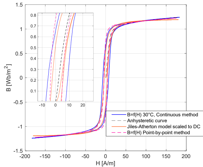
Fig. 5. Magnetisation characteristics – model vs measured at 30°C
