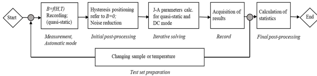
Fig. 4. Schematic diagram of the measurement algorithm used
