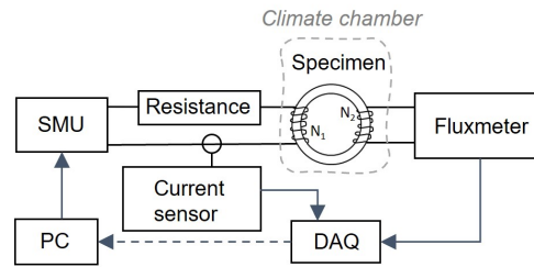
Fig. 2. Schematic diagram of the measurement system used
