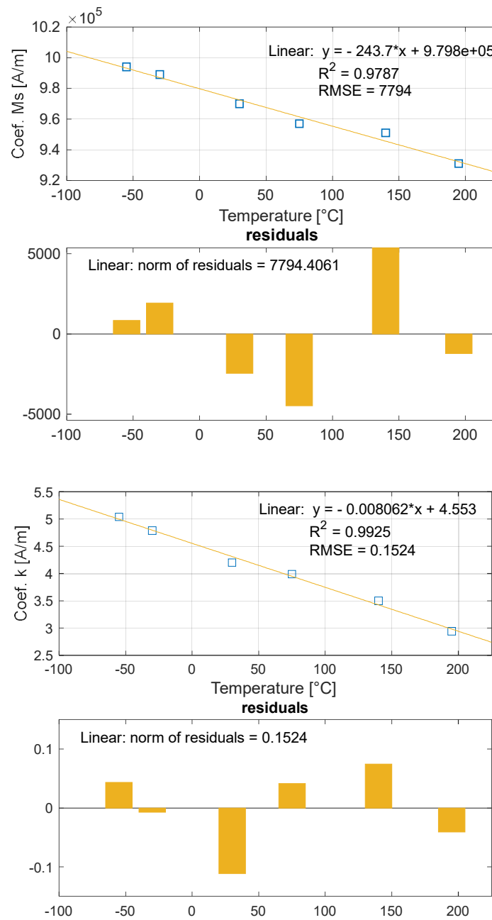
Fig. 18. Linear approximation of the J-A model parameter values for the ASTM A753 Alloy 2 in the temperature range of -55 to 195^\circ\text{C}
