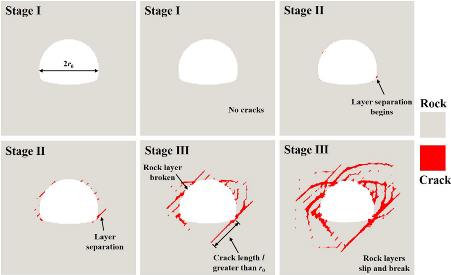
Fig. 11. Evolution of cracks in the surrounding rock
