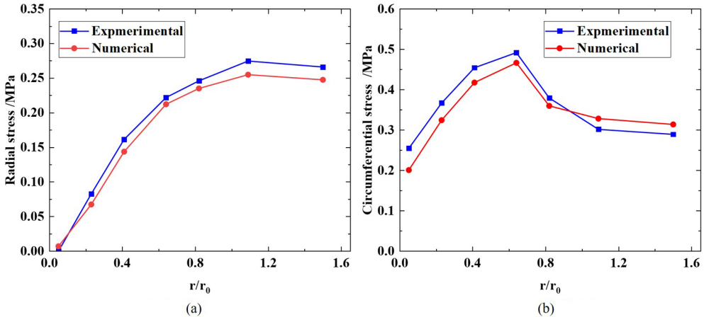
Fig. 6. Comparison between numerical results and experimental data of 45° model under gauge line 2:
