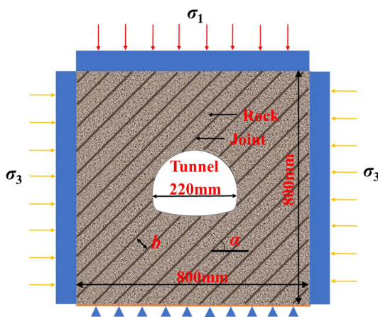
Fig. 8. Geometric model of tunnel loading damage
