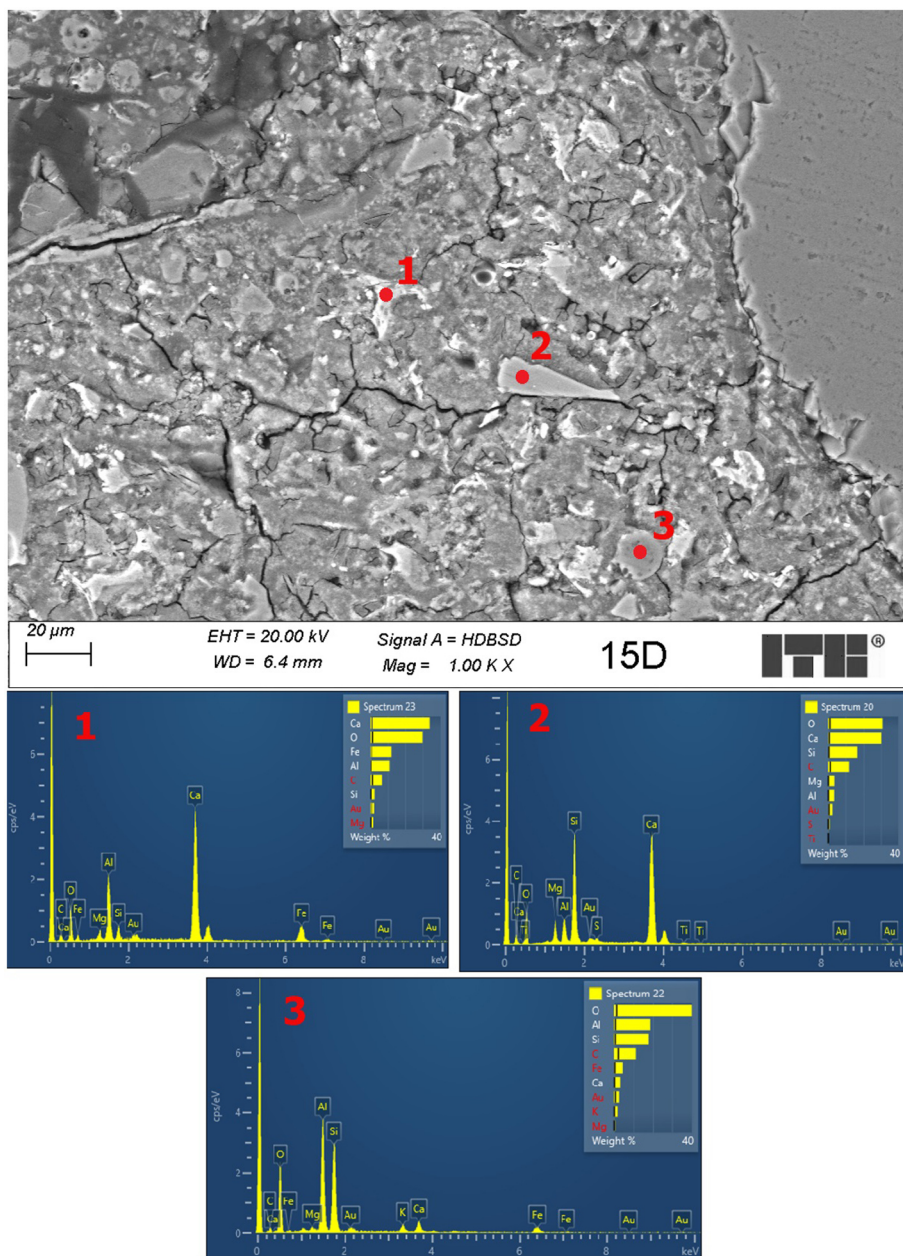
Fig. 6. Sample 15D with identified constituents of cement matrix (1 – clinker, 2 – blast furnace slag, 3 – siliceous fly ash)
