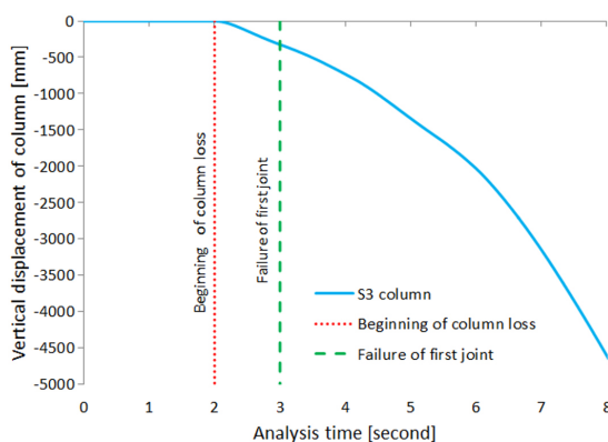
Fig. 4. Vertical displacement of S3 column-analysis time curve for 4B_F/E+3.50 case
