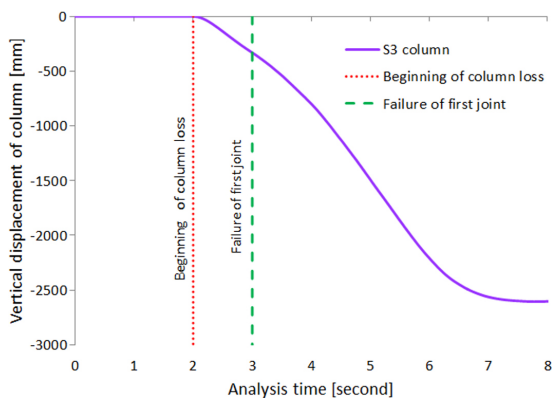
Fig. 7. Curve of vertical displacement of S3 central column vs. analysis time for 4B_F/E+10.50 case
