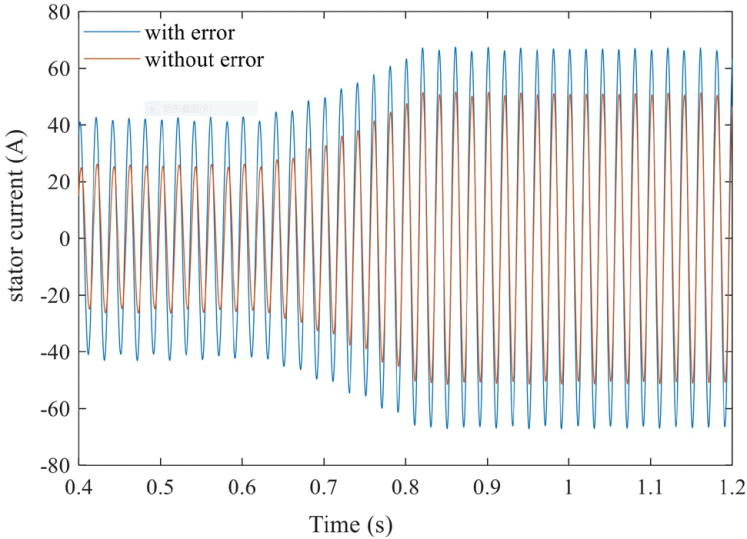
Fig. 21. Time response of stator current under different traction speeds
