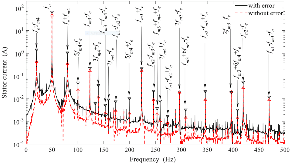
Fig. 23. The spectrum of three-phase stator current when traction speed v_q = 3 m/min
