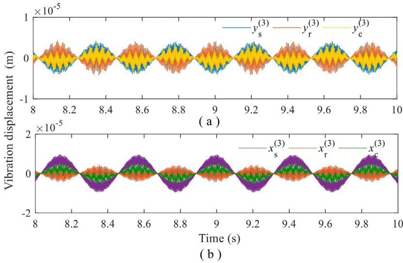
Fig. 11. Vibration displacement time history of sun, ring and carrier for the third stage PGSs: (a) vibration displacement in the y direction, (b) vibration displacement in the x direction
