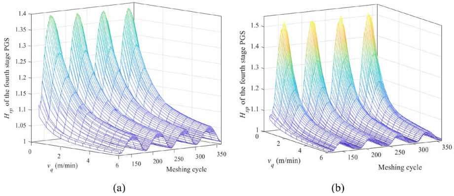
Fig. 18. Distribution rule of LSC in the fourth-stage PGS at different traction speeds, (a) H_{rp} between ring and planet, (b) H_{sp} between sun and planet
