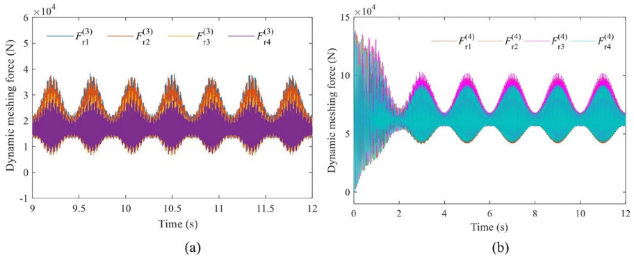
Fig. 13. Dynamic meshing force for planet-ring in two-stage PGSs: (a) meshing force F_m^{(3)} ( n = 1, 2, \dots, N ) for third-stage PGS, (b) meshing force F_m^{(4)} ( n = 1, 2, \dots, N ) for fourth-stage PGS
