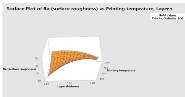
Fig. 5. Surface plot
