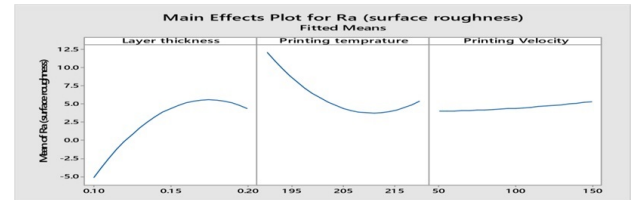
Fig. 3. Main effects plot
