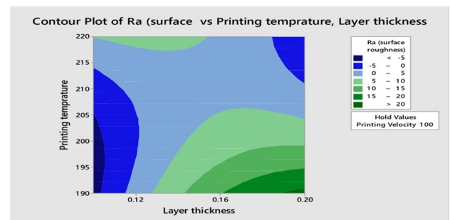
Fig. 4. Contour plot
