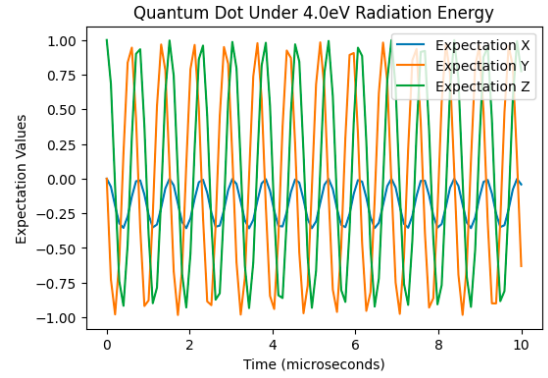
Fig. 4. Plot of expectation value of quantum dot under 4.0eV radiation energy
