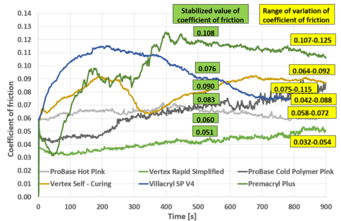
Fig. 10. Sliding friction coefficients of acrylic polymers in artificial saliva
