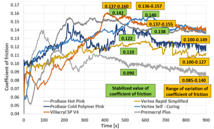
Fig. 9. Sliding friction coefficients of acrylic polymers in physiological saline
