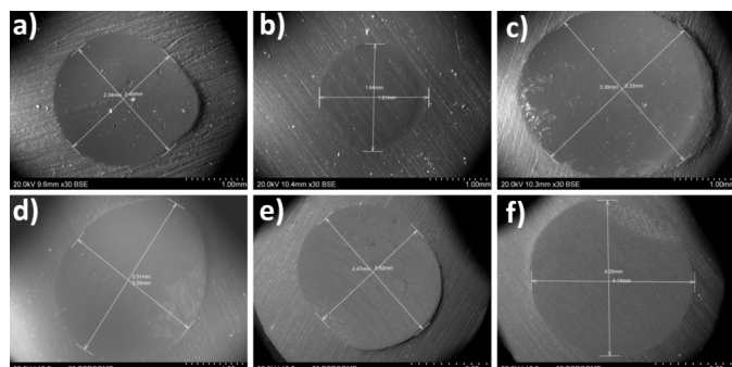
Fig. 6. SEM images of the structure, along with defect measurements, of discs from: (a) ProBase Hot Pink, (b) Vertex Rapid Simplified, (c) ProBase Cold Polymer Pink, (d) Vertex Self Curing, (e) Villacryl SP V4, (f) Premacryl Plus
