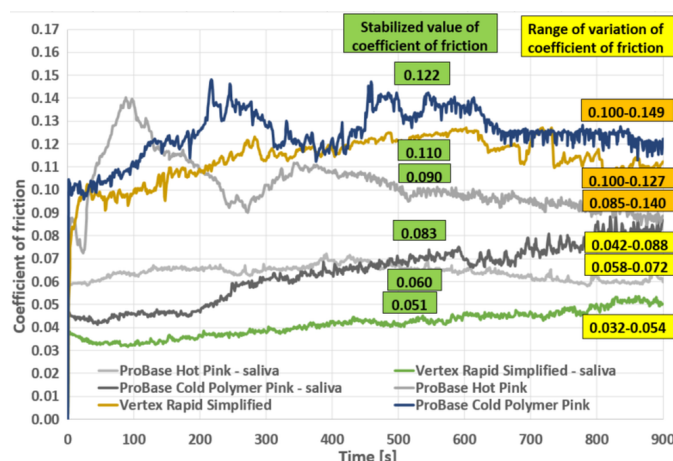
Fig. 12. List of friction coefficients of selected acrylic resins for denture plates in physiological saline and artificial saliva
