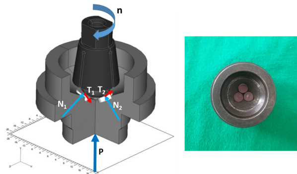
Fig. 4. Spatial system of forces in the friction node and a set of 3 discs after the test
