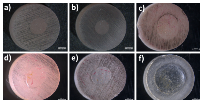
Fig. 5. Optical microscopy images of the structure of the surface layer in the defect of discs from: (a) ProBase Hot Pink, (b) Vertex Rapid Simplified, (c) ProBase Cold Polymer Pink, (d) Vertex Self Curing, (e) Villacryl SP V4, (f) Premacryl Plus
