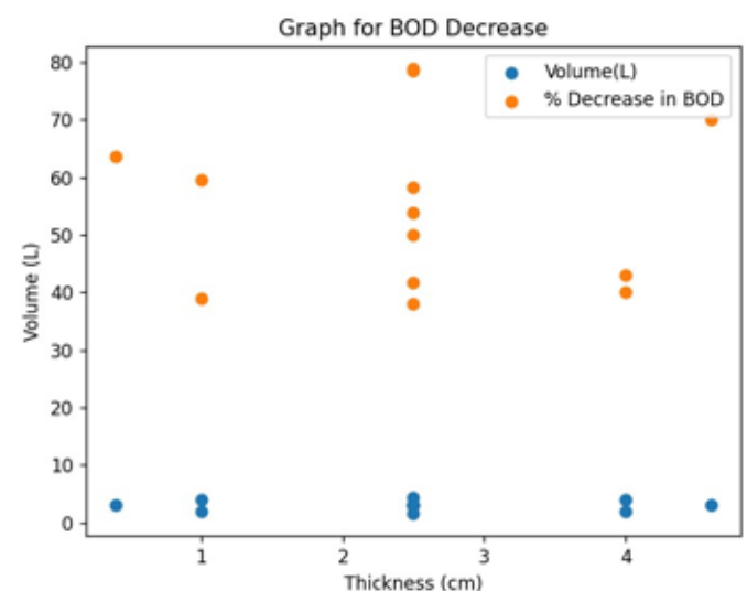
Fig 7. Reduction of BOD for different thicknesses of hair substrate and volume of sample in constructed wetland.
