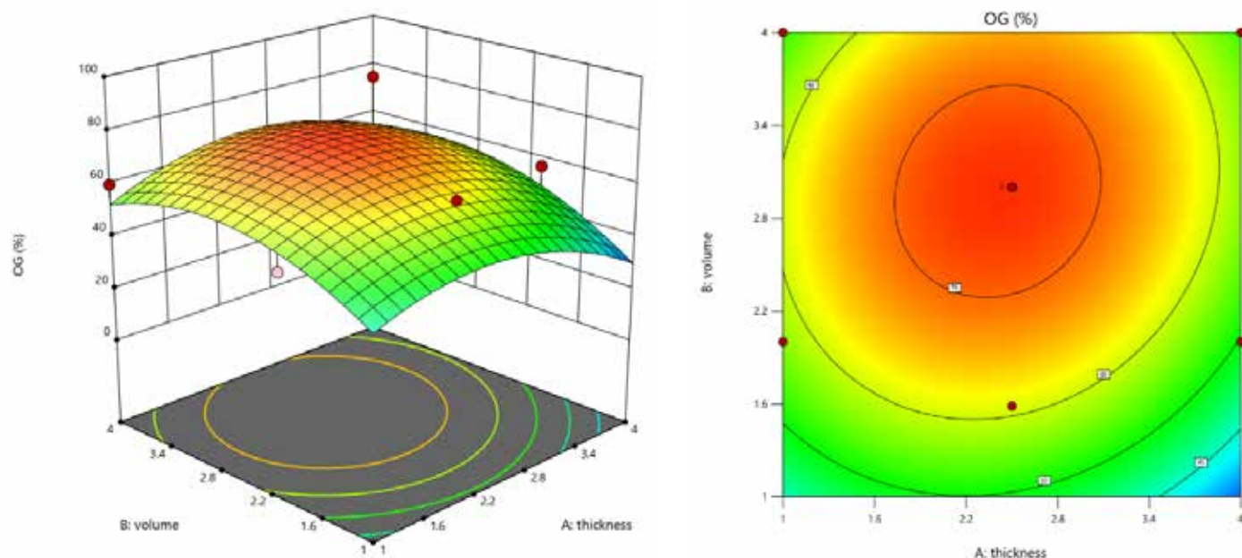
Fig 4. Surface and contour plot for Oil & Grease removal of adsorption using human hair, obtained from RSM studies
