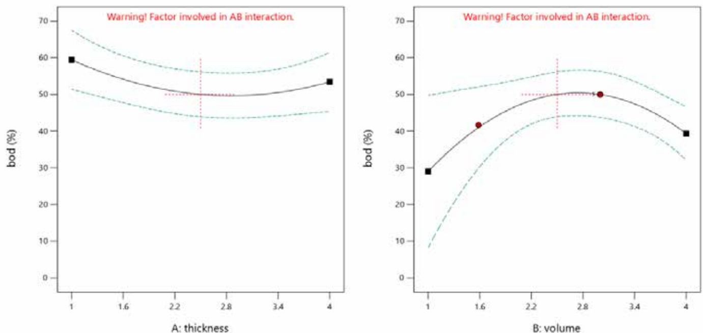
Fig 3. Effect of thickness and volume on BOD decrease by using human hair. Data obtained from RSM studies.
