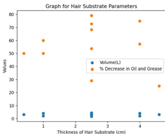
Fig 6. Reduction of oil and grease for different thicknesses of hair substrate and volume of sample in a constructed wetland.
