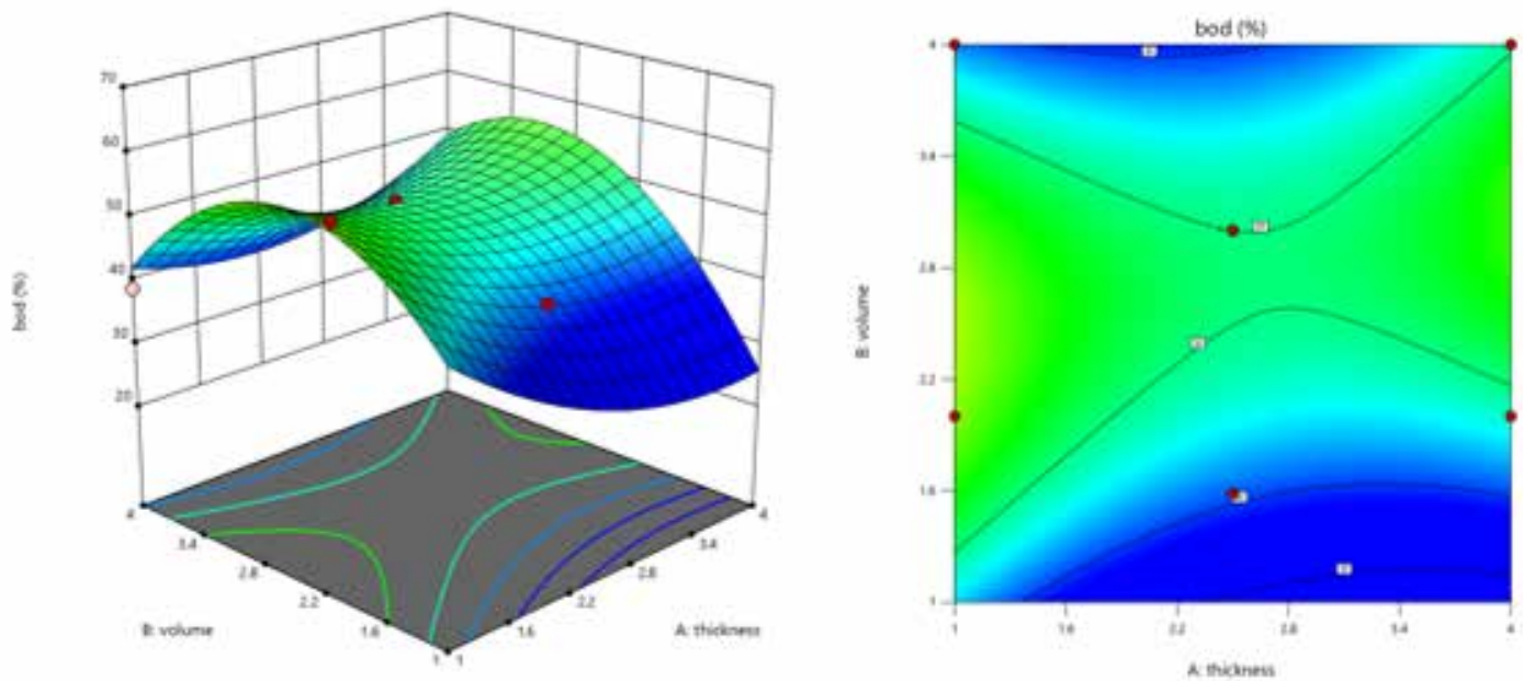
Fig 2. Surface and contour plot for BOD decrease of adsorption using human hair, obtained from RSM studies
