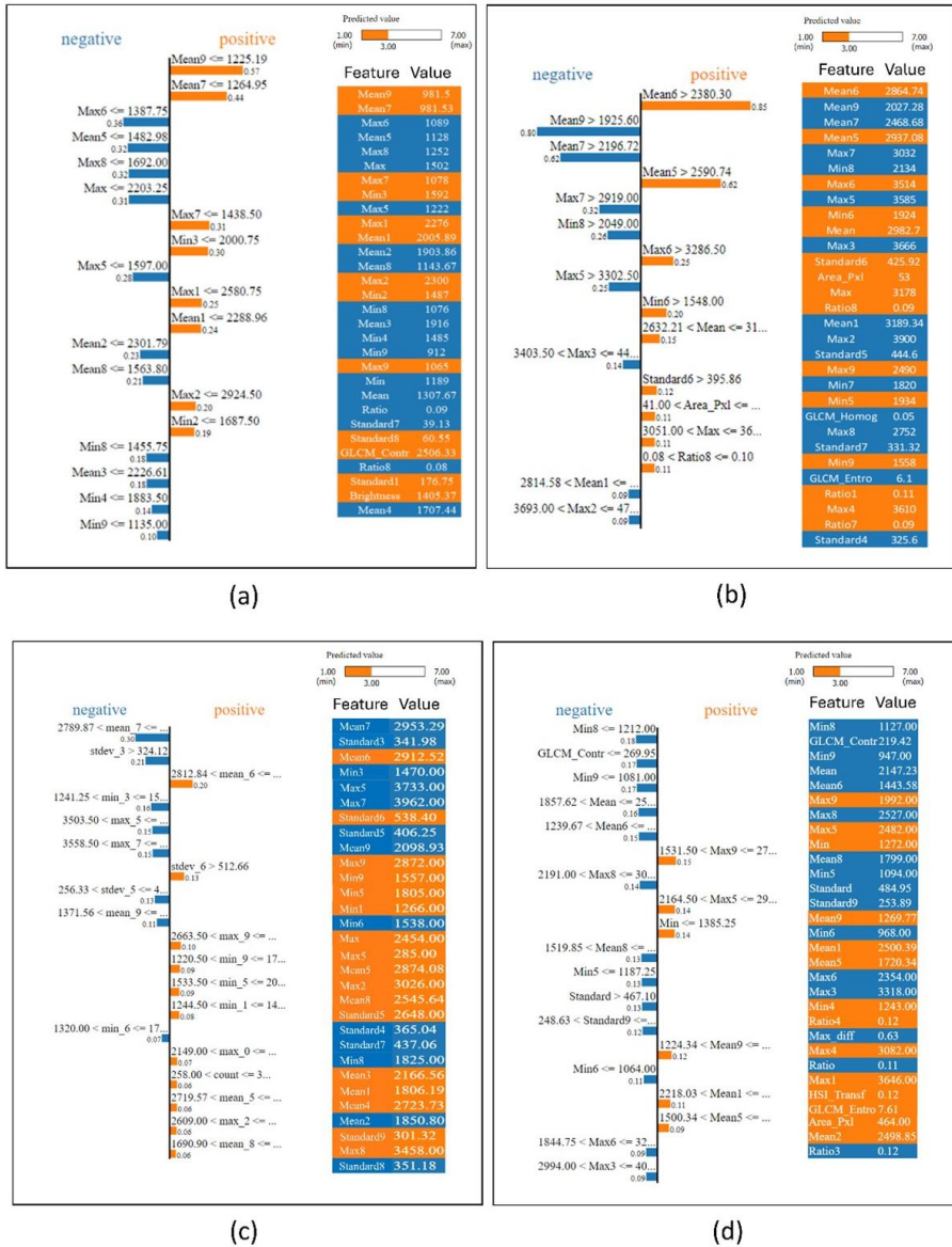
Fig. 6. LIME graphs for classifications using (a) MRS, (b) SLIC, (c) Mean shift and (d) Quick Shift segmentations. Note that the numbers next to the features in OBIA represent the bands used. For example, features without numbers (such as max, ratio, min) were calculated using the blue band. Features marked '2' are used for the green band, '3' for the red band, '4-5-6' for the red-edge bands, '7' for the NIR band, '8' for the narrow NIR band and '9-10' for the SWIR bands
