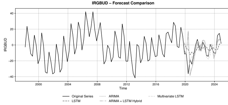
Figure 7: Comparison of IRGBUD model results for sensitivity analysis.
