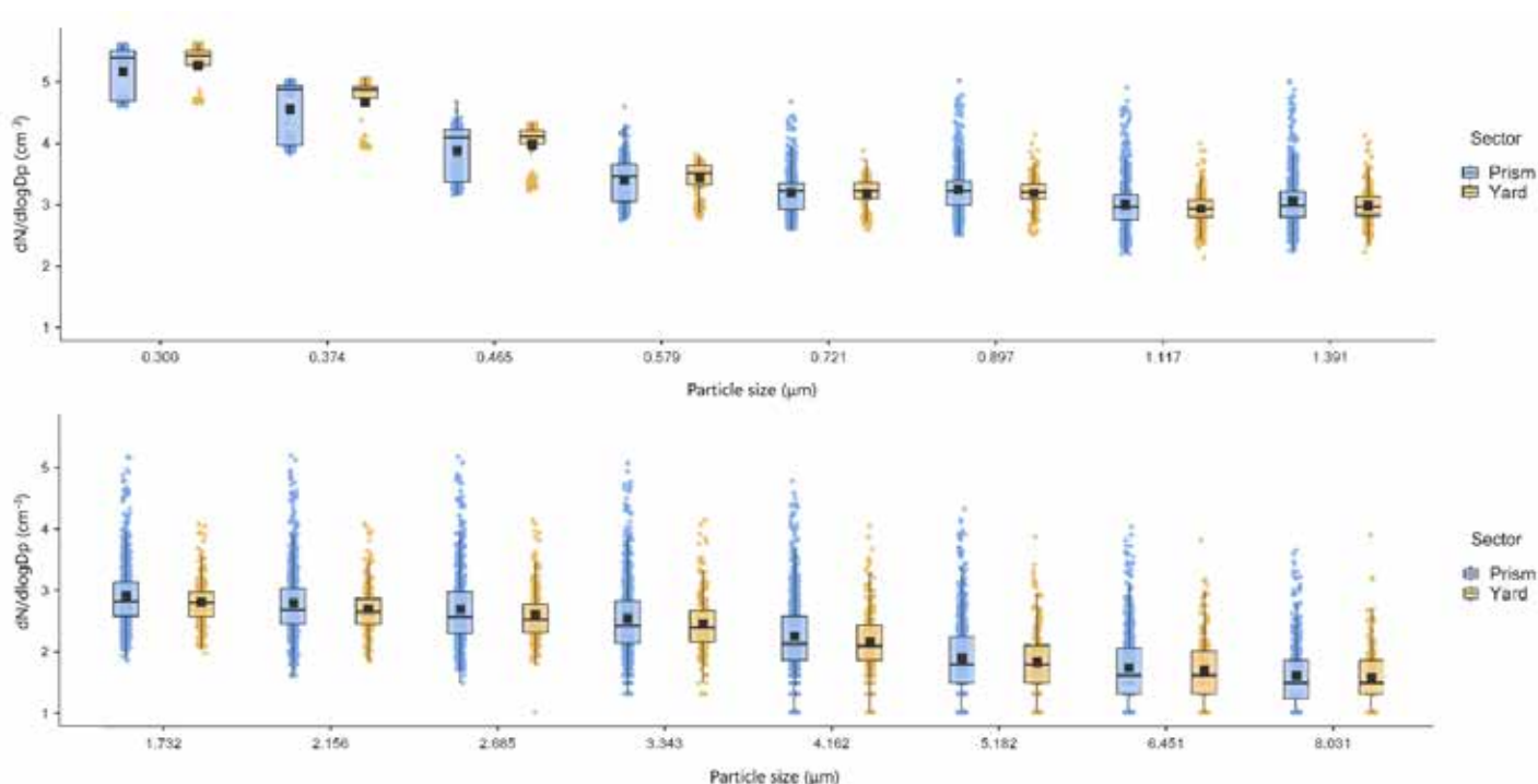
Figure 4. Particle number size distribution (logarithmic scale), expressed as dN/d\log D_p [ \text{cm}^{-3} ], by sampling sector. a) Particles sized 0.300-1.391 \mu\text{m} ; b) Particles sized 1.732-8.031 \mu\text{m} .
