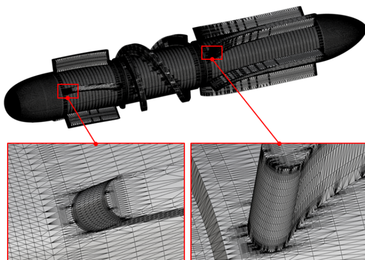
Fig. 8. Node-to-node triangular mesh of axial blood pump
