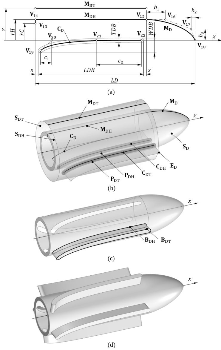
Fig. 5. Diffuser modelling
