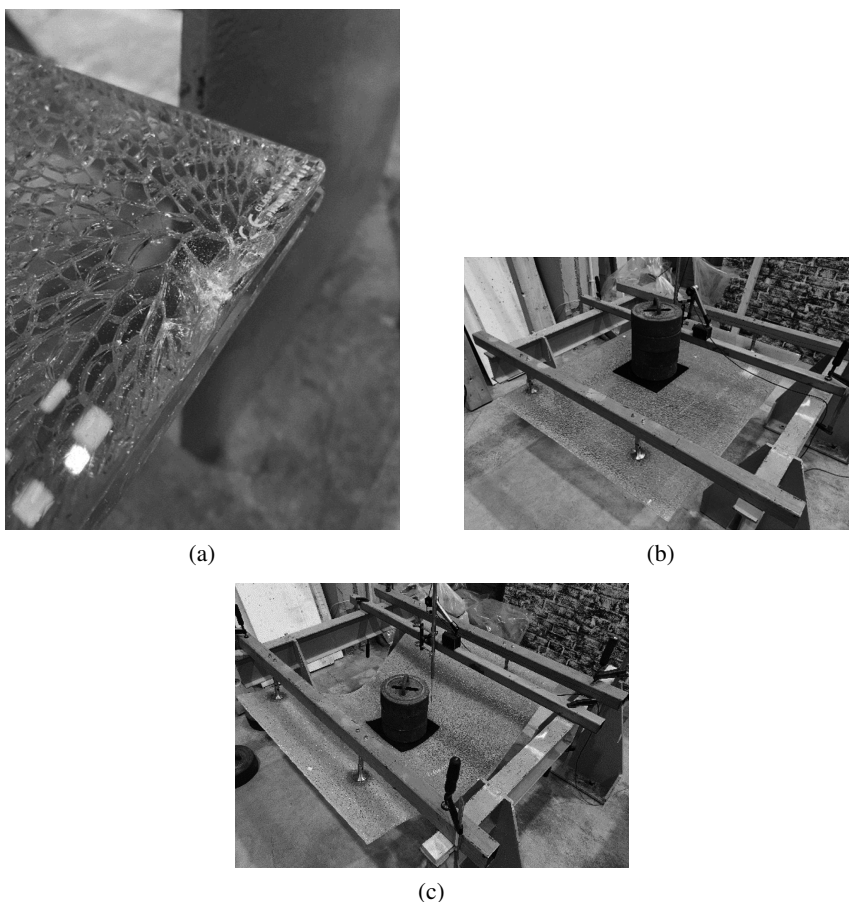
Fig. 8. Real-scale sample experiments: (a) fracture location, (b) sample subjected to point loading, (c) sample after loading of 0.75 kN maintained for 120 hours
