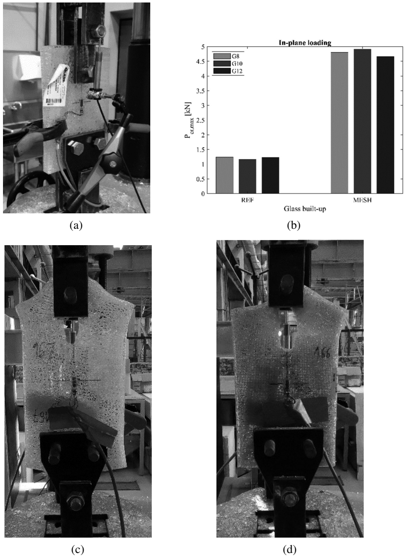
Fig. 3. In-plane loading: (a) test set-up, (b) results, (c) ultimate failure of reference sample, (d) ultimate failure of reinforced sample
