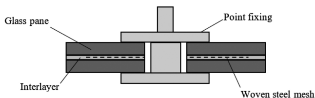
Fig. 1. Reinforcement of the area around the opening (patent application for the invention "Localized reinforcement of laminated glass" in UPRP No. P.437856)
