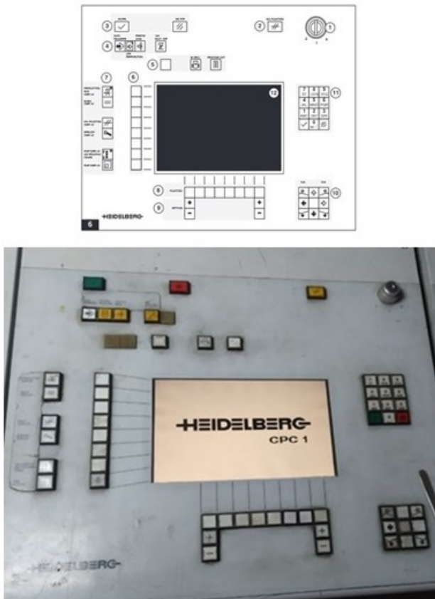
Fig. 4. CPC 1.04 control panel, the only IIoT gathering point for information analyses on SM74-4P 1997, source: own elaboration based on (Heidelberg, 1997)
