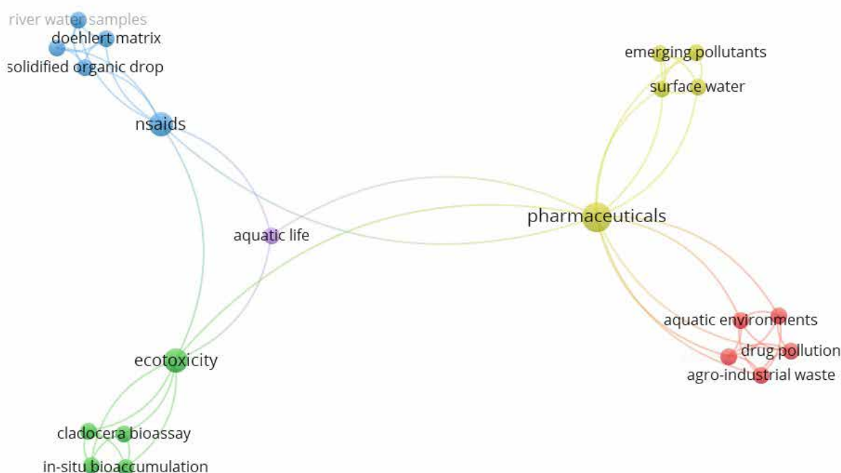
Fig. 2. Network map generated from keywords of articles searched in SCOPUS based on words: NSAIDs AND pollution AND water; map was prepared in VOSviewer software.
