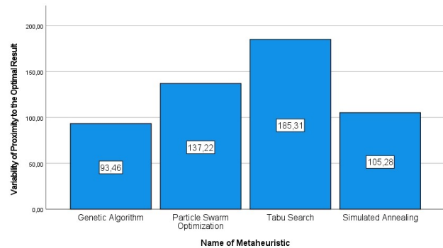
Fig. 2. Variability of Proximity to the Optimal Result for each Metaheuristic
