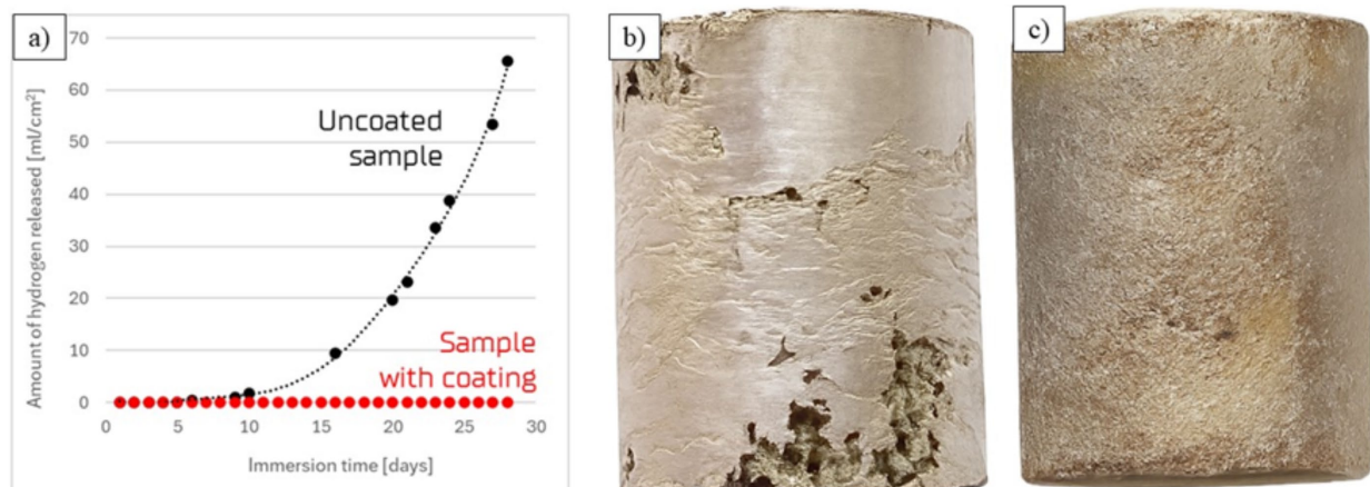
Fig. 11. The graph presenting comparison of hydrogen evolution during incubation of uncoated and conversion-coated samples a) and the images of the sample after the immersion test: b) sample without coating and c) sample with coating after 28 days in immersion corrosion test
