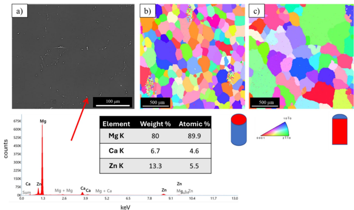
Fig. 4. SEM/BSE image with exemplary EDS spectrum a), and SEM/EBSD orientation maps of the MgZn1Ca0.2Li1 from cross sections of the as-cast ingot b), c)
