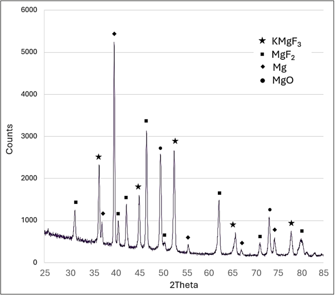
Fig. 5. XRD diffraction pattern of the MgZn1Ca0.2Li1 alloy with conversion coating
