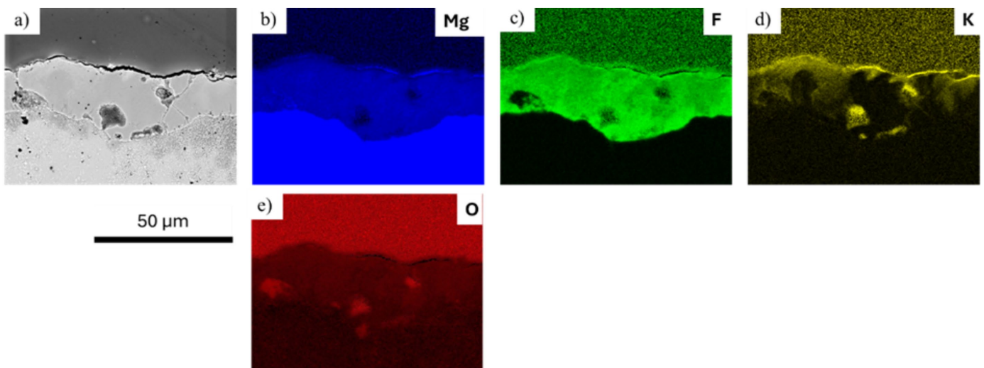
Fig. 7. SEM/EDS analysis of the conversion coating: a) SEM/BSE cross-sectional image of the analyzed area, b) magnesium, c) fluorine, d) potassium, e) oxygen
