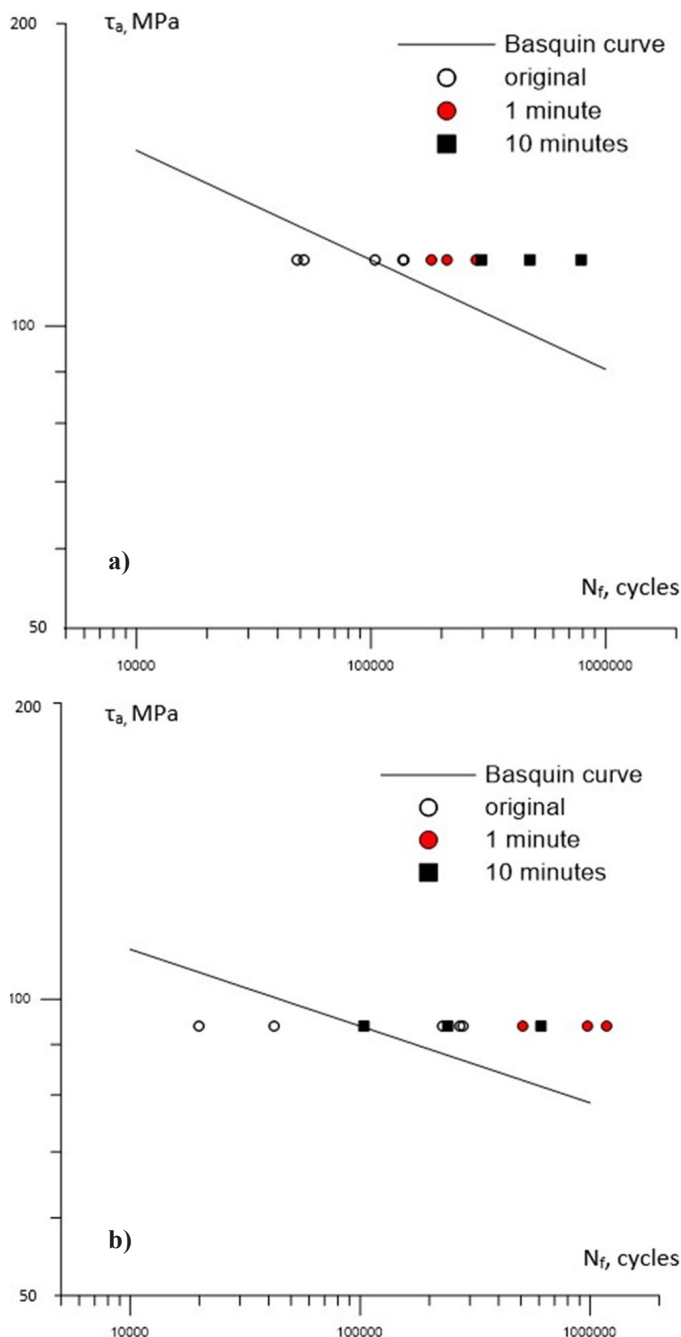
Fig. 10. Summary of nominal fatigue characteristics for cyclic torsion along with experimental points when strengthened by vibratory shot peening: a) T6, b) T64
