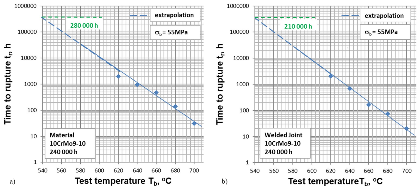
Fig. 7. Results of short creep tests of welded joint materials of the secondary steam pipeline after 240 000 h of operation under creep conditions in the form of the relation \log t_{re} = f(T_b) at \sigma_b = 55 MPa
