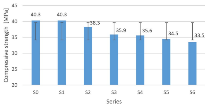
Fig. 6. Average compressive strength after 28 days
