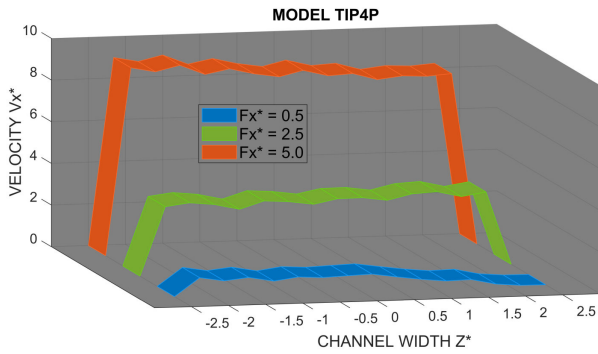
Fig. 12. Velocity distribution in a copper nanochannel in the direction of flow (60 molecules of water – model TIP4P, time interval 30–50 ps)
