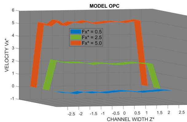
Fig. 6. Velocity distribution in a copper nanochannel in the direction of flow (60 molecules of water – model OPC, time interval 30–50 ps)
