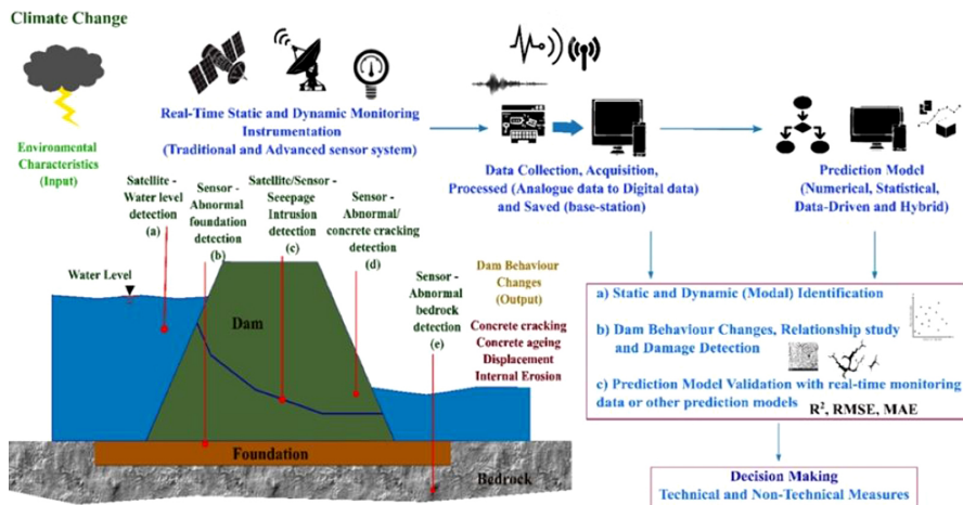
Fig. 2. The comprehensive Structural Health Monitoring (SHM) System for monitoring the static and dynamic properties of concrete dams
