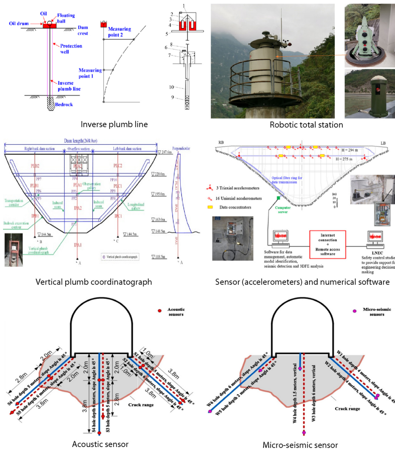
Fig. 3. Example of the ground-based monitoring tools [23, 57–59, 65]
