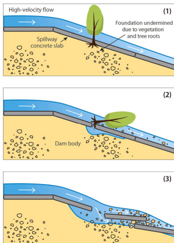
Toddbrok Dam incident: Poor maintenance, high velocity flow, material degradation
