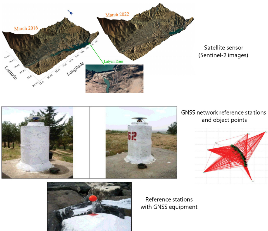
Fig. 4. Example of the space-based monitoring tools [40, 62]
