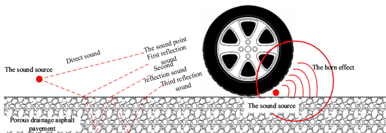
Fig. 3. Tire and ground noise propagation
