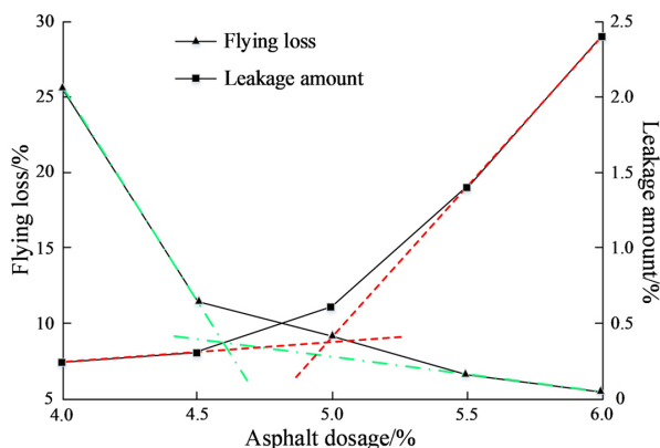
Fig. 2. The optimum asphalt dosage range of PAC-13 (VV = 23%)
