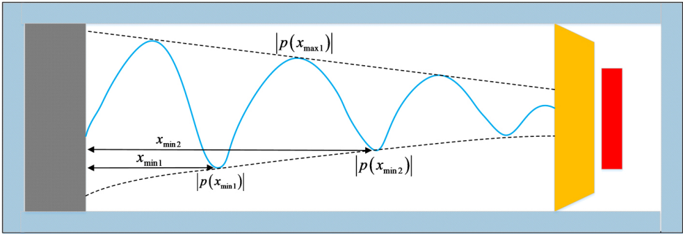
Fig. 4. Standing wave diagram of standing wave tube test
