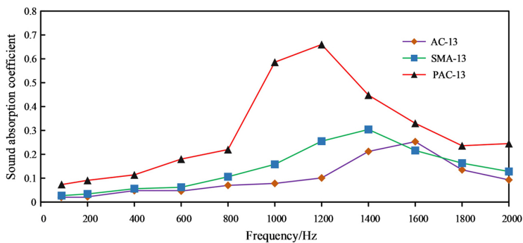
Fig. 5. Sound absorption coefficient of specimens with different frequencies
