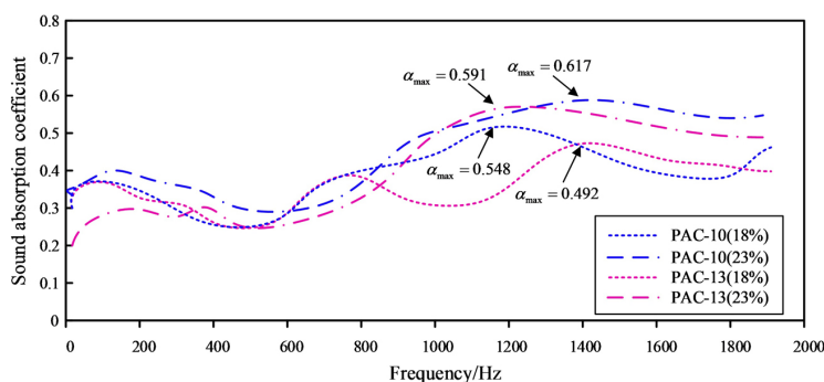
Fig. 8. Spectrum diagram of acoustic absorption coefficient of PAC with different particle sizes
