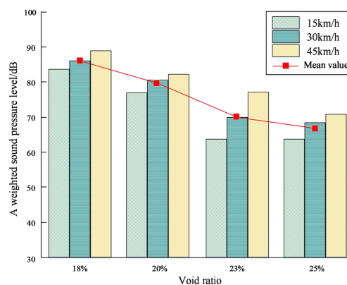
Fig. 7. Average noise sound pressure level of PAC-13
