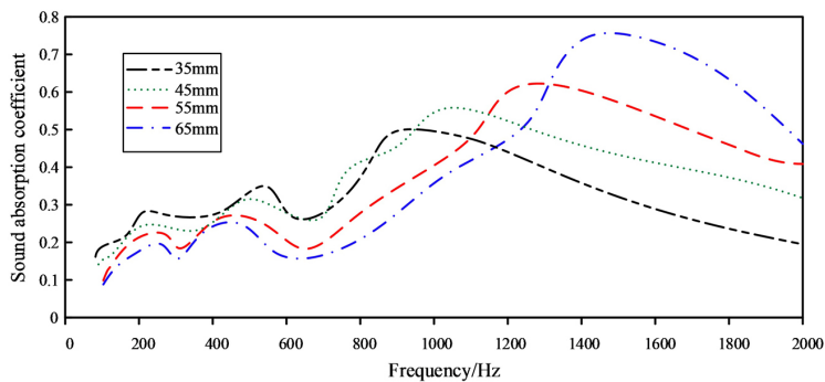
Fig. 6. Spectrum diagram of sound absorption coefficient of PAC-13 with different thickness
