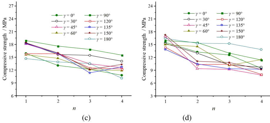
Fig. 5. Influence of n on the uniaxial compressive strength of the specimens for selected \gamma and \beta : (a) \beta = 30^\circ ; (b) \beta = 45^\circ ; (c) \beta = 60^\circ ; (d) \beta = 75^\circ
