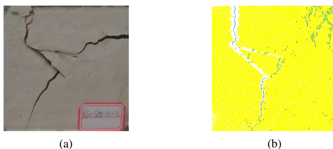
Fig. 6. Comparison of experiment results and numerical simulation of the failure characteristics of the rock mass specimens with dentate discontinuity
