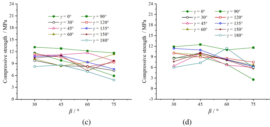
Fig. 8. Influence of various \beta on the numerical simulation results of the uniaxial compressive strength of the rock mass specimens for selected n and \gamma : (a) n = 1 ; (b) n = 2 ; (c) n = 3 ; (d) n = 4
