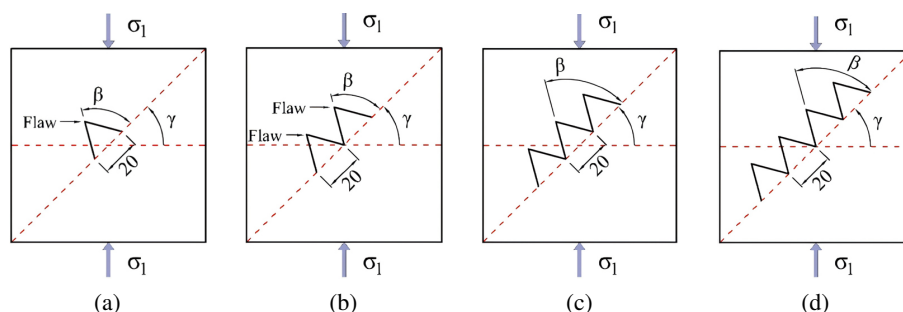
Fig. 1. Schematic diagram of uniaxial compression for specimens with regular dentate discontinuity: (a) n = 1 ; (b) n = 2 ; (c) n = 3 ; (d) n = 4
