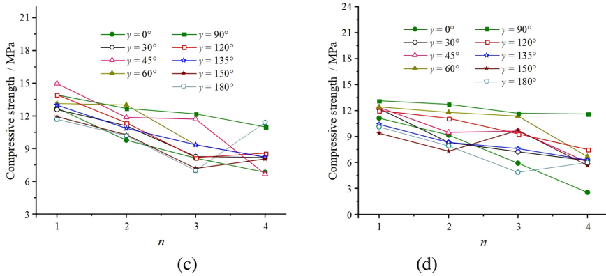
Fig. 9. Influence of various n on the numerical simulation results of the uniaxial compressive strength of the rock mass specimens for selected \gamma and \beta : (a) \beta = 30^\circ ; (b) \beta = 45^\circ ; (c) \beta = 60^\circ ; (d) \beta = 75^\circ
