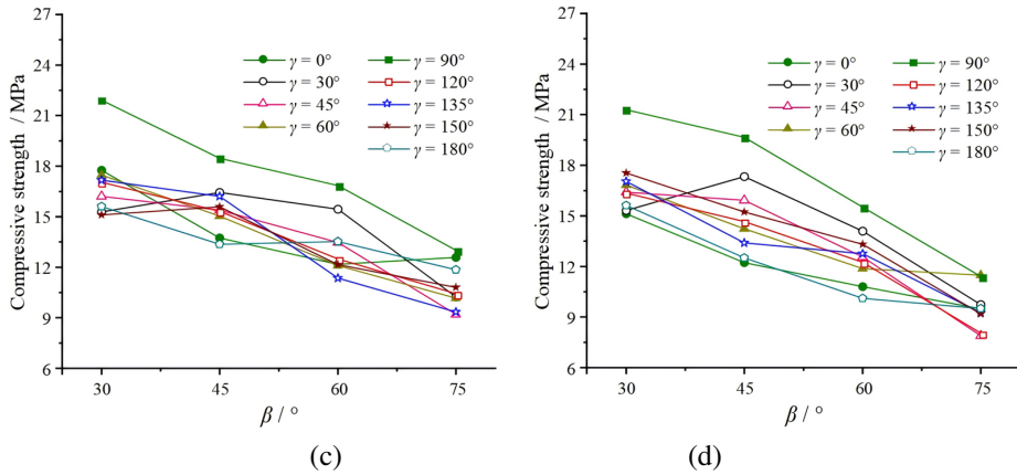
Fig. 4. Influence of various \beta on the uniaxial compressive strength of the specimens for selected n and \gamma : (a) n = 1 ; (b) n = 2 ; (c) n = 3 ; (d) n = 4
