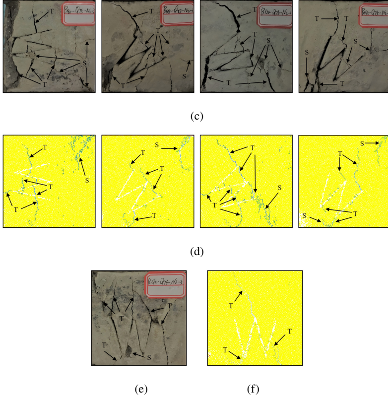
Fig. 10. Influence of various \gamma on the failure characteristics of the rock mass specimens in the experiments and numerical simulations when n = 2 and \beta = 75^\circ . In the panels, T and S represent tensile and shear cracking: (a) \gamma = 0^\circ , \gamma = 30^\circ , \gamma = 45^\circ , \gamma = 60^\circ ; (b) \gamma = 0^\circ , \gamma = 30^\circ , \gamma = 45^\circ , \gamma = 60^\circ ; (c) \gamma = 90^\circ , \gamma = 120^\circ , \gamma = 135^\circ , \gamma = 150^\circ ; (d) \gamma = 90^\circ , \gamma = 120^\circ , \gamma = 135^\circ , \gamma = 150^\circ ; (e) \gamma = 180^\circ ; (f) \gamma = 180^\circ
