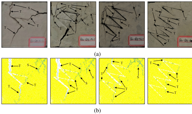
Fig. 12. Influence of various n on the failure characteristic of the rock mass specimens in the experiments and numerical simulations when \beta = 75^\circ and \gamma = 60^\circ : (a) n = 1, n = 2, n = 3, n = 4 ; (b) n = 1, n = 2, n = 3, n = 4
