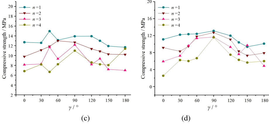
Fig. 7. Influence of various \gamma on the numerical simulation results of the uniaxial compressive strength of the rock mass specimens for each selected n and \beta : (a) \beta = 30^\circ ; (b) \beta = 45^\circ ; (c) \beta = 60^\circ ; (d) \beta = 75^\circ
