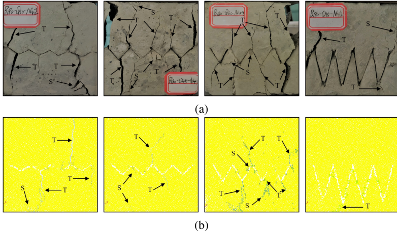
Fig. 11. Influence of various \beta on the failure characteristic of the rock mass specimens in the experiments and numerical simulations when n = 4 and \gamma = 180^\circ : (a) \beta = 30^\circ, \beta = 45^\circ, \beta = 60^\circ, \beta = 75^\circ ; (b) \beta = 30^\circ, \beta = 45^\circ, \beta = 60^\circ, \beta = 75^\circ
