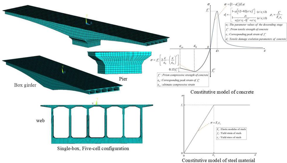
Fig. 5. Finite element model of Bridge
