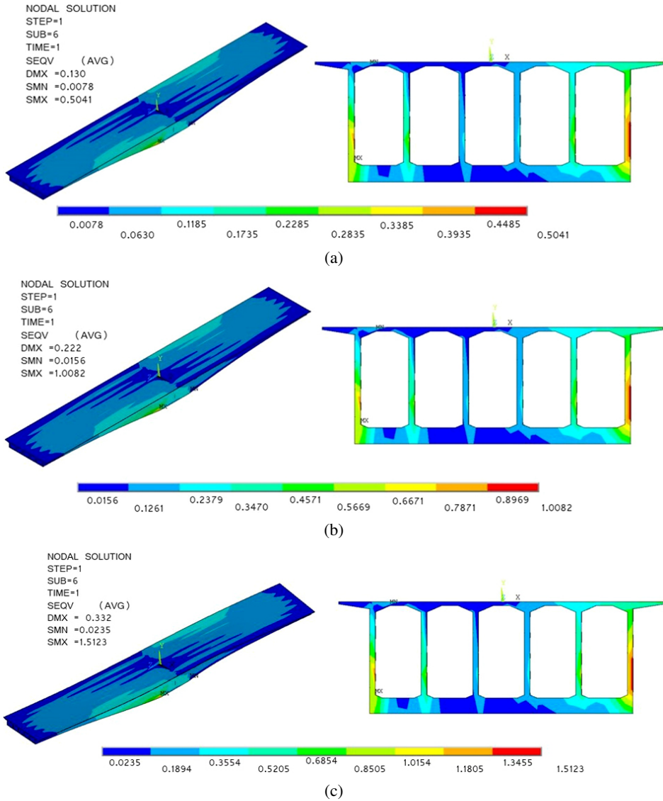
Fig. 8. Stress of PC girder under varying rotary acceleration (Unit: MPa): (a) 1.00 \times 10^{-3} \text{ rad/min}^2 ; (b) 2.00 \times 10^{-3} \text{ rad/min}^2 ; (c) 3.00 \times 10^{-3} \text{ rad/min}^2
