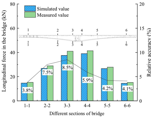
Fig. 11. Longitudinal force under uniform rotating
