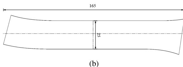
Fig. 1. Layout of background bridge (Unit: m): (a) Prototype bridge layout diagram; (b) Prototype bridge top view
