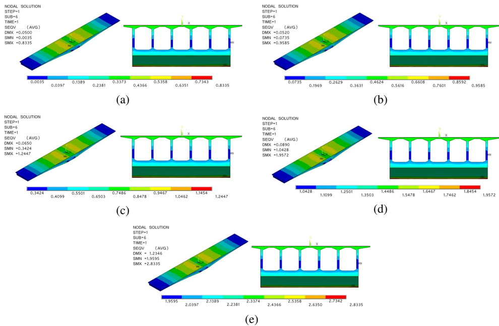
Fig. 7. Numerical prediction of bridge models with rotational angular velocities and gravity (Unit: MPa): (a) 0.01 rad/min; (b) 0.015 rad/min; (c) 0.02 rad/min; (d) 0.05 rad/min; (e) 0.10 rad/min
