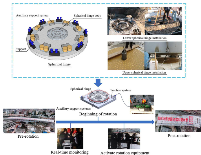
Fig. 2. Configuration of rotation system
