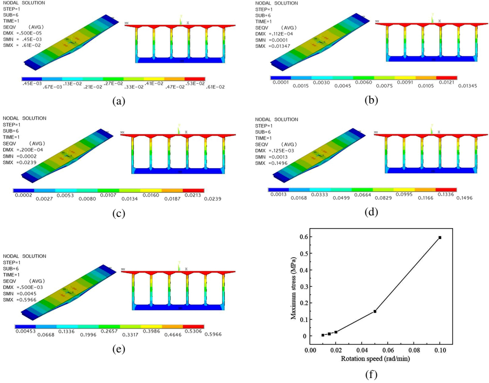
Fig. 6. Numerical prediction of bridge models with rotational angular velocities (Unit: MPa): (a) 0.01 rad/min; (b) 0.015 rad/min; (c) 0.02 rad/min; (d) 0.05 rad/min; (e) 0.10 rad/min; (f) Relationship between rotation speed and the maximum stress
