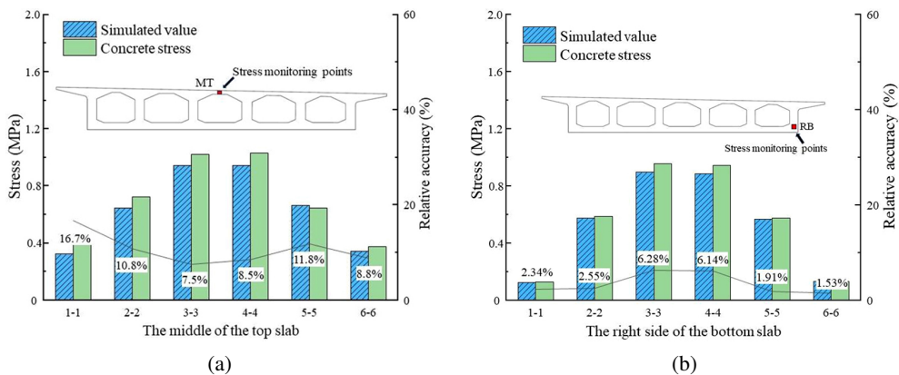
Fig. 10. Comparison of the measured value and simulated value: (a) Uniform rotating stage; (b) Acceleration rotating stage
