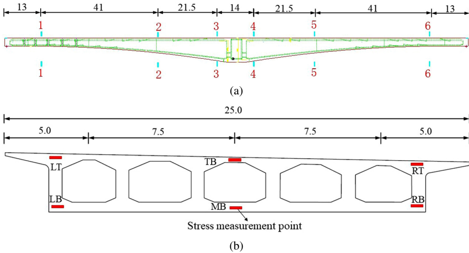
Fig. 4. Measurement arrangement (Unit: m): (a) Arrangement of critical sections; (b) Distribution of strain sensors
