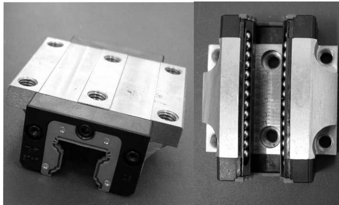
Fig. 1. Studied rail system Mannesmann Rexroth, catalogue number 1651.25
