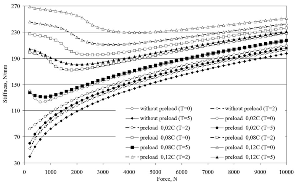
Fig. 10. Characteristics of stiffness of the block-rail system, with parallelism errors, with at preload force perpendicular to the mounting surface of the runner block
