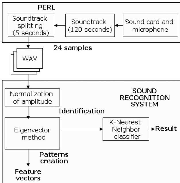
Fig. 1. Process of sound recognition of induction motor with the use of eigenvector method and K-Nearest Neighbor Classifier
