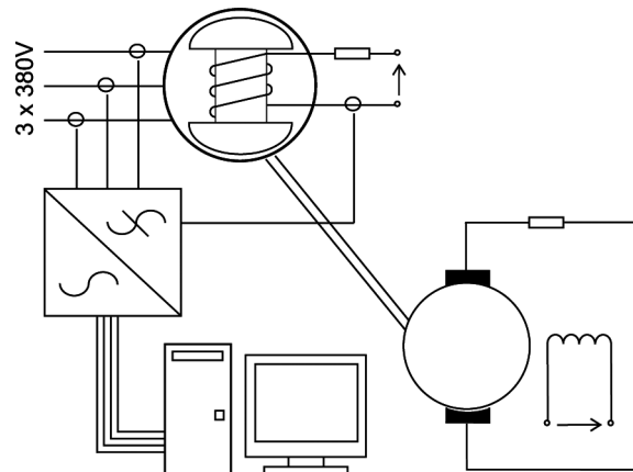
Fig. 2. Schematic diagram of the measuring stand
