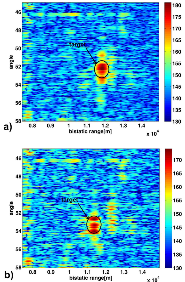
Fig. 11. Results of ground clutter removal for registered data for: a) first Tx antenna beam scan, b) second TX antenna beam scan.
