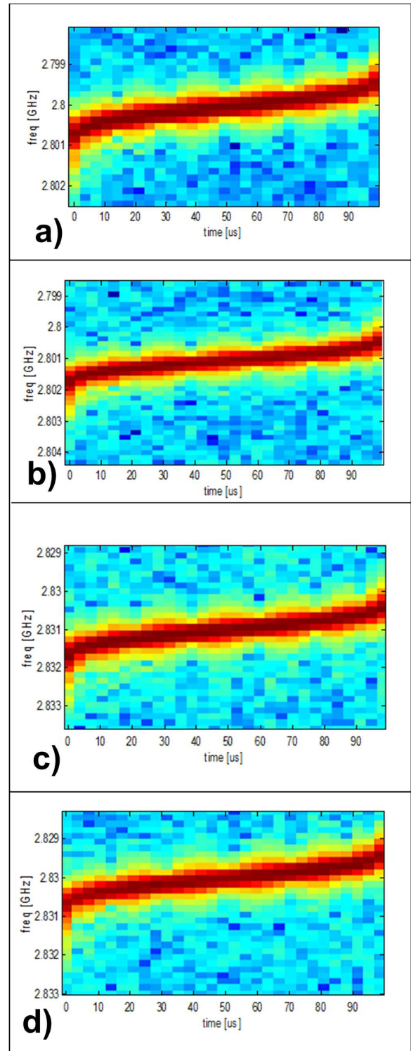
Fig. 9. The internal structure of the transmitted pulses at four different carrier frequencies ( f_c ) – time-frequency plots, color coded in dB: a) f_c = 2.8GHz , b) f_c = 2.801GHz , c) f_c = 2.831GHz , d) f_c = 2.830GHz .
