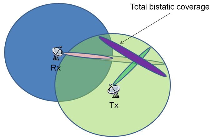
Fig. 3. The simplified geometry for the bistatic pulse radars using mechanically scanning transmitting and receiving antennas: illustration of the range extension for the bistatic radar in comparison to the monostatic case.
