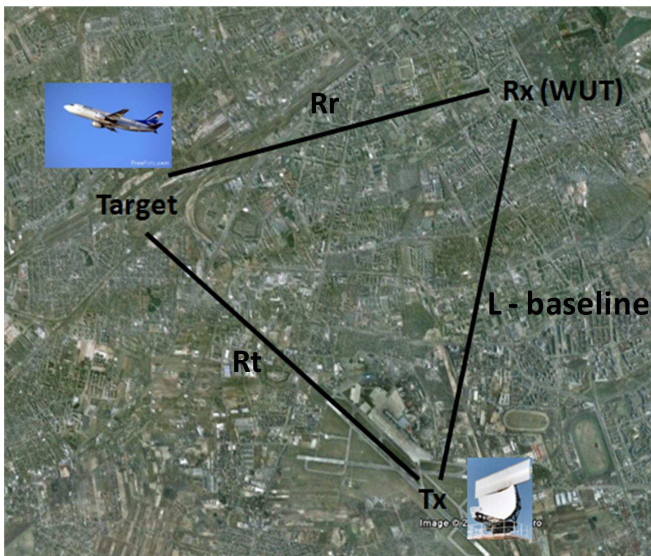
Fig. 4. Simplified bistatic geometry of WUT trials on non-cooperative bistatic radar.
