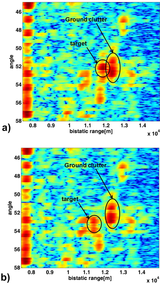
Fig. 10. Results of matched filtering for registered data for: a) first Tx antenna beam scan, b) second TX antenna beam scan.
