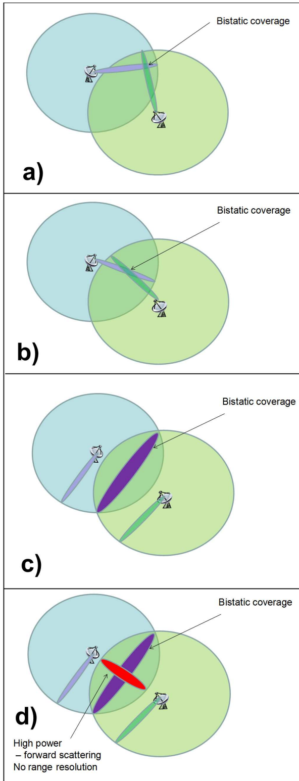
Fig. 2. The simplified geometry for the bistatic pulse radars using mechanically scanning transmitting and receiving antennas: a) bistatic coverage for t = t_1 , b) bistatic coverage for t = t_2 , c) total bistatic coverage, d) total bistatic coverage with marked area of no range resolution.
