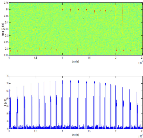
Fig. 8. Transmitted pulse bursts: time frequency plot (upper picture) and time plot (bottom picture).
