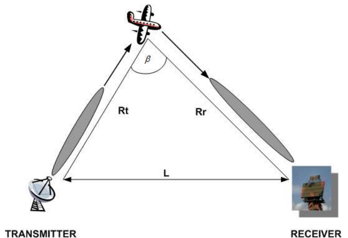
Fig. 1. Simplified bistatic radar geometry.
