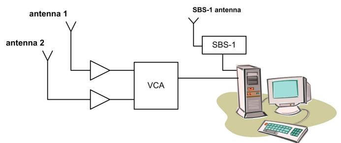
Fig. 6. Simplified block diagram of receiver system used for WUT trials on non-cooperative bistatic radar.
