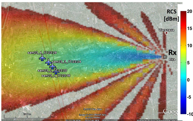
Fig. 5. Map of minimum detectable RCS for simplified bistatic geometry of WUT trials on non-cooperative bistatic radar.
