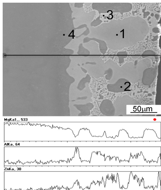
Fig. 4. SEM image of the Mg specimen after heat treatment in contact with the Al+20% Zn powder mixture and the element distribution along the index line
