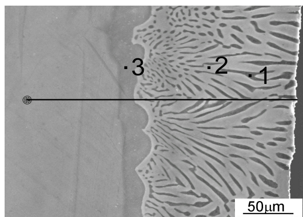
Fig. 1. A corner of the Mg specimen with Al-enriched layer
