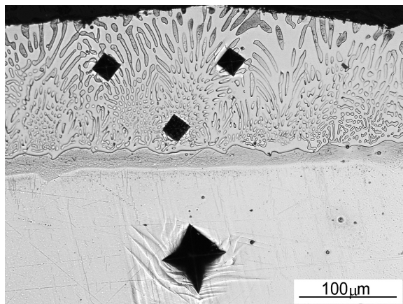
Fig. 3. Microhardness measurement indentations in the Al-enriched layer and the Mg substrate
