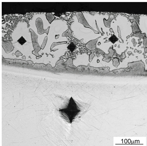
Fig. 5. Microhardness measurement indentations in Al/Zn-enriched layer and Mg substrate
