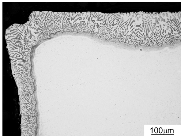
Fig. 1. A corner of the Mg specimen with Al-enriched layer
