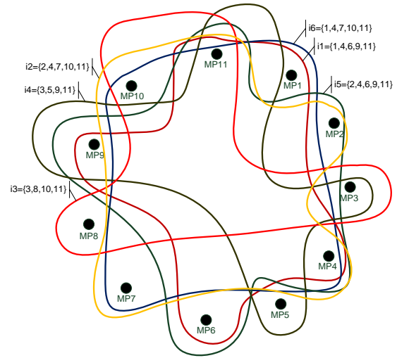
Fig. 6. Non-concurrency hypergraph.
