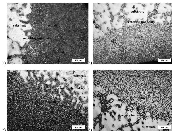
Fig. 5. Microstructures after remelting: a) by laser – AZ91 alloy, b) by GTAW method – AM60 alloy, c) and d) by modified GTAW method, for the AZ91 and AM60 alloys, respectively; optical microscope, etched
