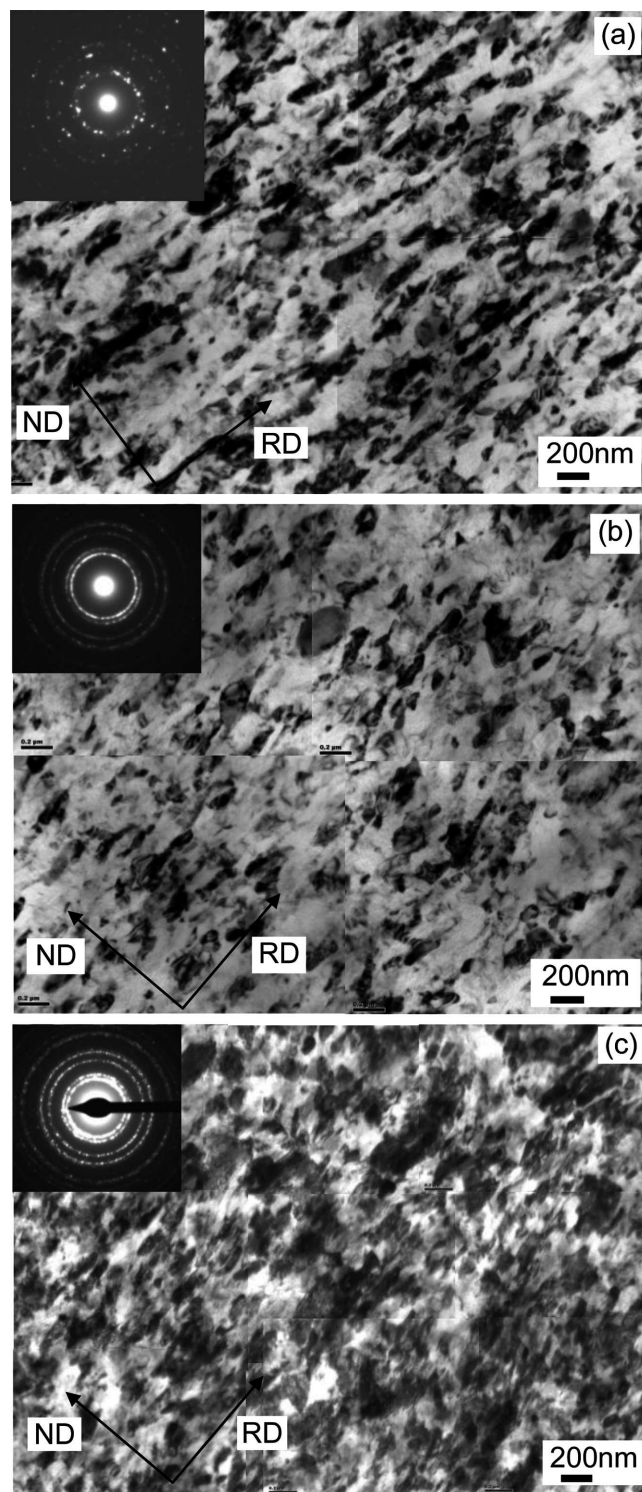
Fig. 3. Microstructure evolution with increasing strain. TEM bright field images observed after: (a) 2, (b) 6 and (c) 10 turns, under 2 GPa pressure. Thin foils cut-out from sample periphery in ND-RD section
