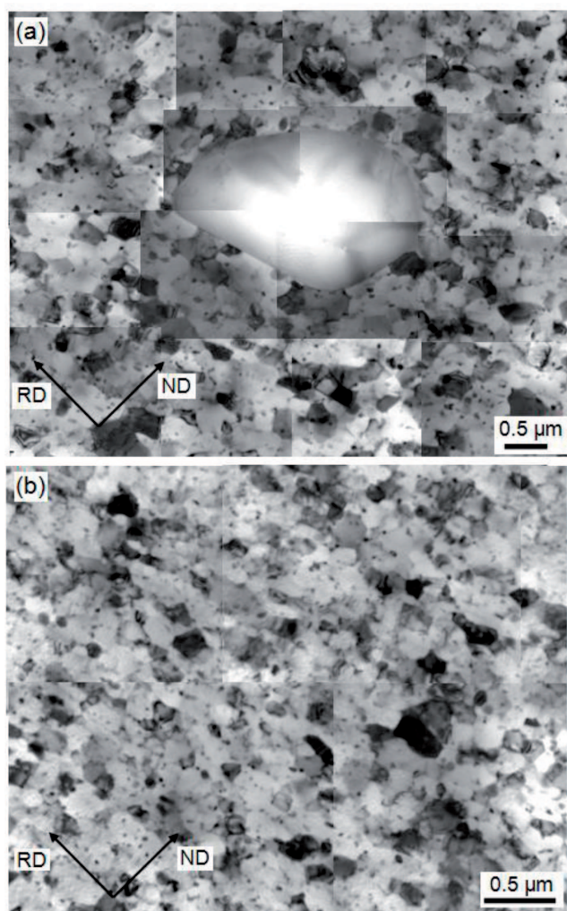
Fig. 8. TEM bright field images showing microstructures after recrystallization at 300°C for 60 s. Peripheral region (a) close to and (b) far from SPPs
