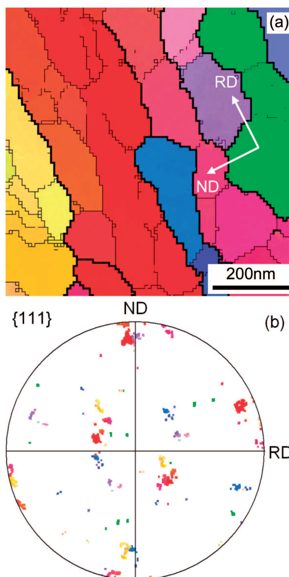
Fig. 9. (a) TEM orientation map and (b) corresponding \{111\} pole figure measured in the axial area of the sample. The sample processed in one turn under 2 GPa pressure and then annealed at 300°C for 30 s. TEM local orientation measurements with step size of 20 nm in ND-RD section. IPF colour code was applied
