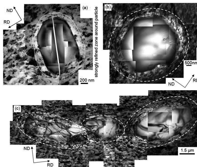
Fig. 6. Microstructures showing the formation of highly deformed zones near large SPPs. Samples deformed under 2 GPa after: (a) – 2 and (b) – 10 turns. (c) Clustering of highly deformed zones observed in the sample deformed under 3 GPa pressure after 4 turns. TEM bright field imaging. Dotted lines indicate strongly deformed zones around large particles
