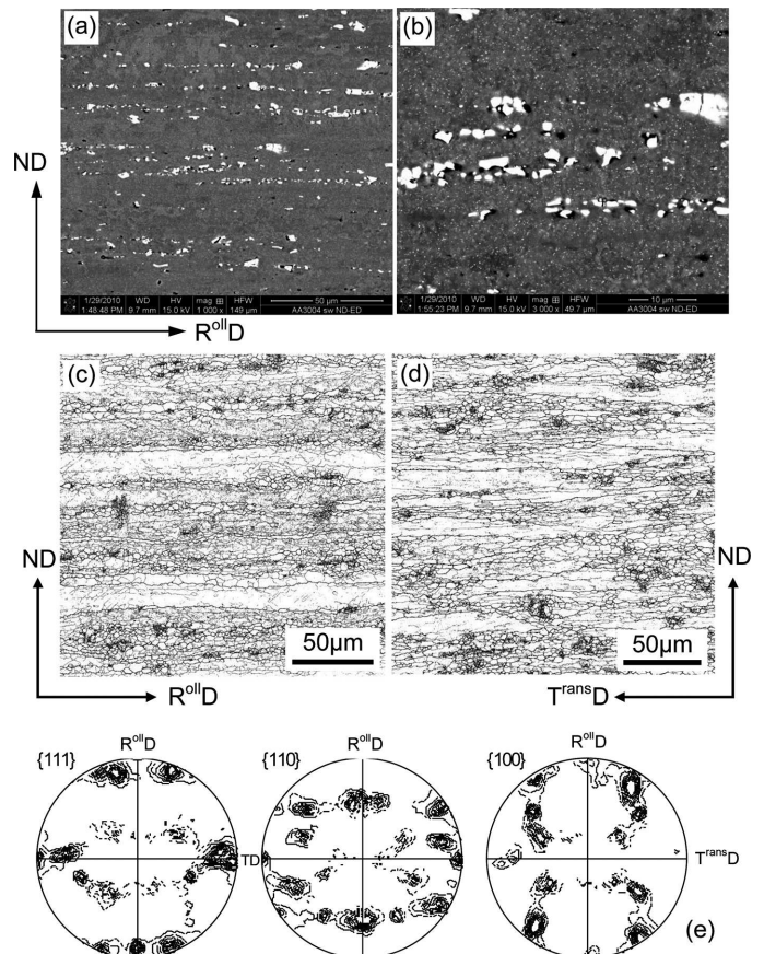
Fig. 2. Initial microstructure of the AA3104 alloy before HPT processing. (a) Layers of large SPPs and (b) randomly distributed dispersoids. SEM imaging in secondary electrons. Grain boundary orientation maps (the boundaries with disorientation angle >1.5^\circ and >15^\circ are marked) showing microstructure of flat grains observed in: (c) ND-R 0 D and (d) ND-T trans D sections and corresponding (e) texture presented in rolling plane. SEM/EBSD local orientation measurements with step size of 100 nm
