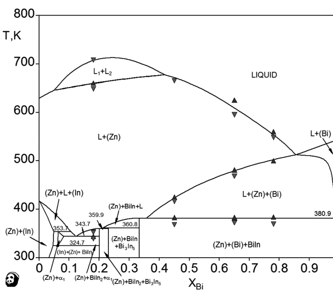
Fig. 9. Vertical section of Bi-In-Zn system for: a) Bi:In = 1:1; b) Bi:In = 1:3; c) Bi:Zn = 1:1; d) In:Zn = 1:1. The experimental DTA signals registered during cooling, ▼, and heating, ▲, cycles were superimposed
