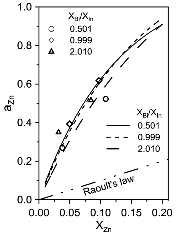
Fig. 6. The zinc activity data obtained from results of Yokokawa et al. [1] at 625 K for six ternary alloys for the Zn composition from 0 to 11 at. % compared with calculated
