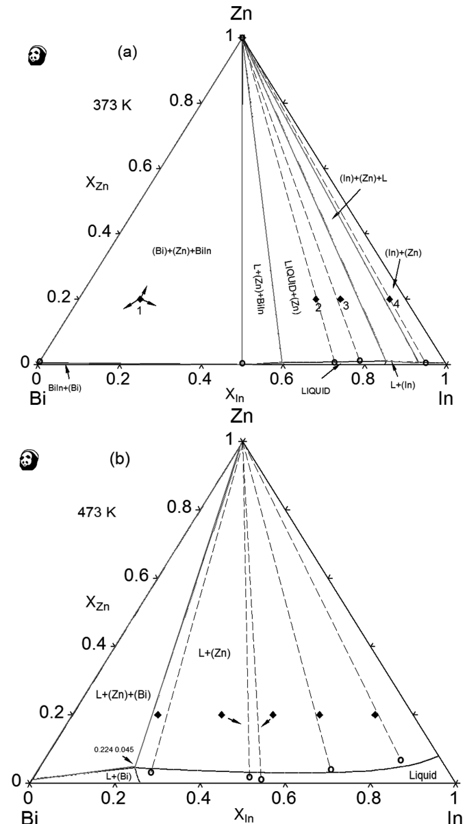
Fig. 8. Isothermal sections of ternary Bi-In-Zn system calculated at: (a) 373 K and (b) 473 K. The experimental data for the solubility of the components in some phases at relevant temperatures after isothermal equilibration ( \circ ) (Table 2 and 3) were superimposed together with the nominal alloy compositions ( \blacklozenge )
