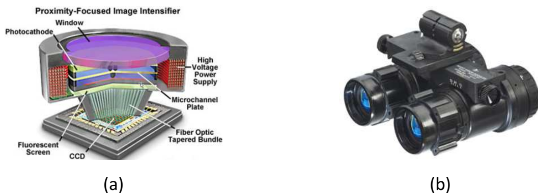
Fig. 15. Night vision device: (a) proximity-focused image intensifier and (b) Gen III night vision goggle AN/AVS-9 (ITT Night Vision).
