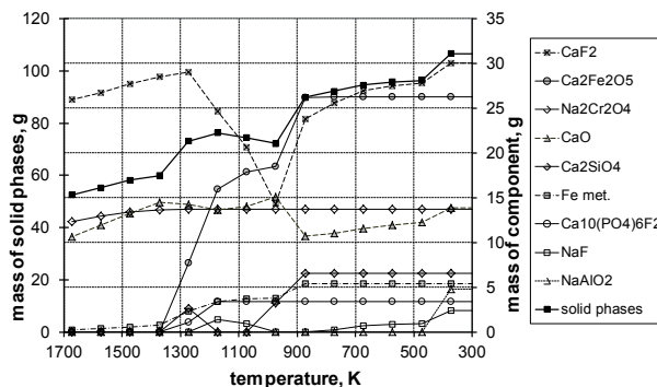
Fig. 2. The course of changes of the mass of the: a) liquid phase; b) solid phase of slag “E” (with cryolite), during solidification of a 106.5g slag sample from a temperature of 1673K down to 298K. At 1673K the mass of the liquid phase of the slag is equal to ca. 54g and the solid phases in the slag is equal to ca. 52.5g
