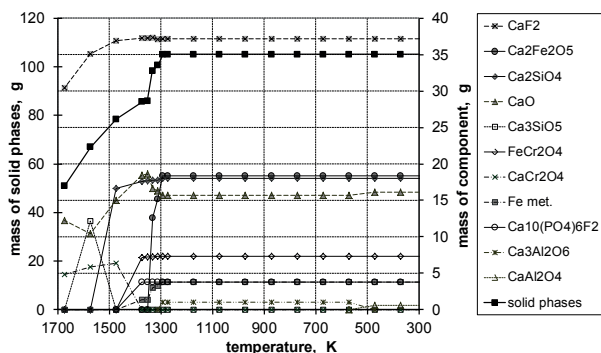
Fig. 1. The course of changes of the mass of the: a) liquid phase; b) solid phase of slag “B” (without cryolite), during solidification of a 105g slag sample from a temperature of 1673K down to 298K. At 1673K, the mass of the liquid phase in the slag is equal to ca. 54g and the solid phases in the slag is equal to ca. 51g
