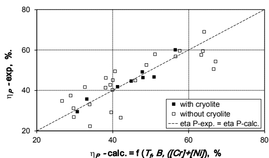
Fig. 4. A comparison of the experimental data of dephosphorization effectiveness with those computed with regression Eqs. (2) and (3)
