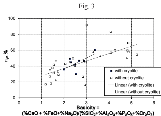
Fig. 3. Dephosphorization effectiveness, \eta_p , as a function of the slag basicity for all heats
