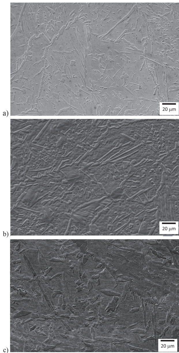
Fig. 3. The microstructure in the duplex stainless S82441 welded at heat input: a) 0.27kJ and shielding gas of 100% Ar, b) 0.43kJ and shielding gas of 85%Ar+15%N 2 , c) 0.72kJ and shielding gas of 50%Ar+50%He
