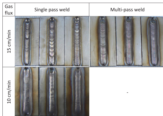
Fig. 5. The TIG welded surface of stainless steel S82441 with single pass weld and multi-pass weld made with filler metal (3 samples for each variant) in the 100% Ar shielding with flux 10 and 15 cm/min in as welded condition
