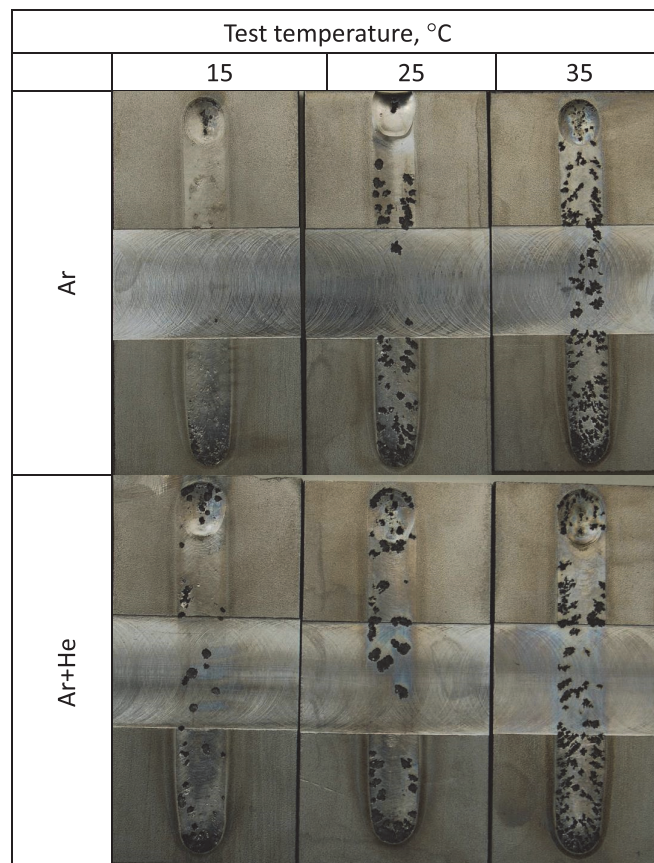
Fig. 14. The autogenous TIG welded joint of stainless steel S82441 made with Ar shielding and Ar+He mixture and welding current of 200A after corrosion test ASTM G48 at temperatures 15, 25 i 35 °C
