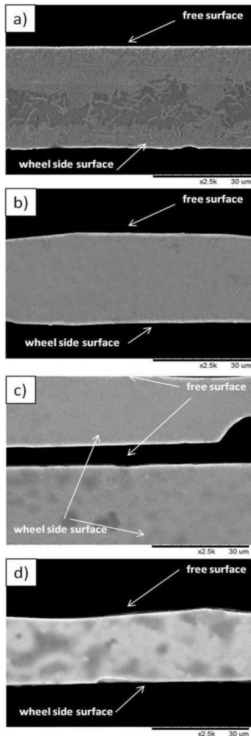
Fig. 11. SEM photos obtained for WE 43 + Cu ribbons with wheel speeds a) 10 m/s, b) 12,5 m/s, c) 15 m/s, d) 17,5 m/s
