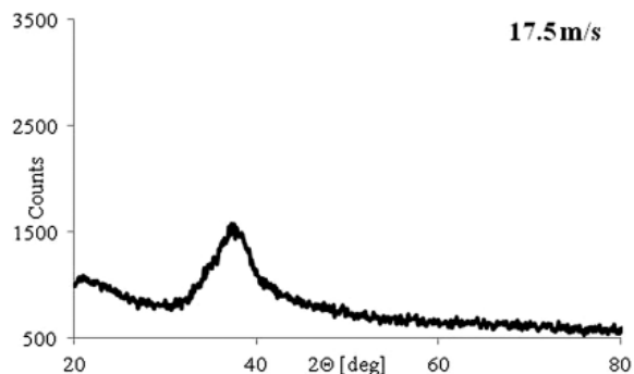
Fig. 8. XRD pattern obtained for WE 43 + Cu ribbons rapidly solidified with wheel speed 17,5 m/s
