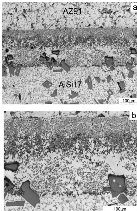
Fig. 1. OM images of the microstructure of the bonding zone formed between AZ91 and AlSi17 by compound casting: (a) lower magnification, (b) higher magnification
