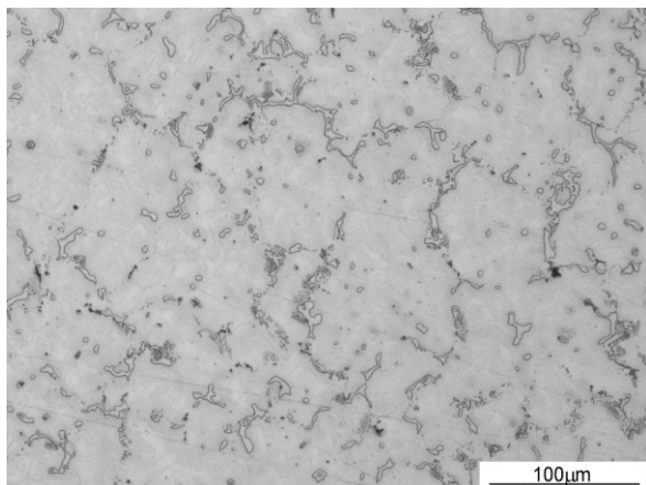
Fig. 5. Microstructure of AZ91 alloy observed at a distance of 500 \mu\text{m} from the bonding zone
