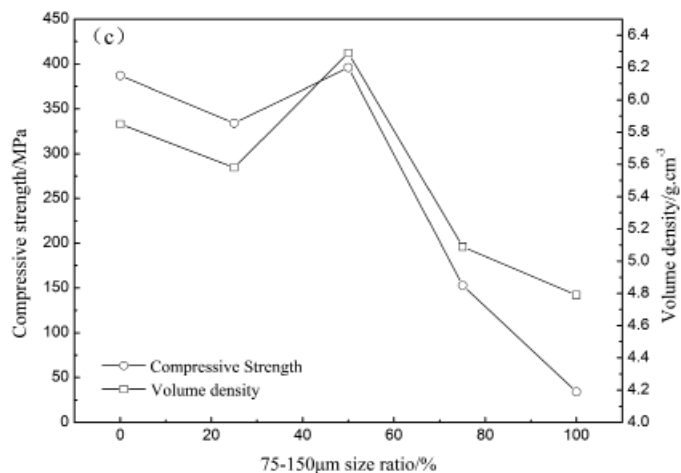
Fig. 6. Effects of (a) sintering temperature, (b) holding time and (c) 75-150 \mu\text{m} size ratio on properties of ferromanganese agglomerates
