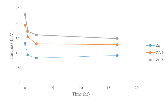
Fig. 8. Variation of microhardness of Zn, ZA1 and ZC2 deposits at 250°C for 0.5, 2 and 16 h.
