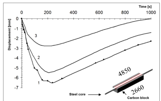
Fig. 6. Changes in the displacement of pin ends during cooling of cast iron in the shaped groove examined for the section preheated to a temperature of T_N = 200^\circ\text{C} and T_N = 350^\circ\text{C} ; 1 – the displacement determined empirically for T_N = 200^\circ\text{C} , 2 – the displacement determined numerically for T_N = 200^\circ\text{C} , 3 – the displacement determined empirically for T_N = 350^\circ\text{C} .
