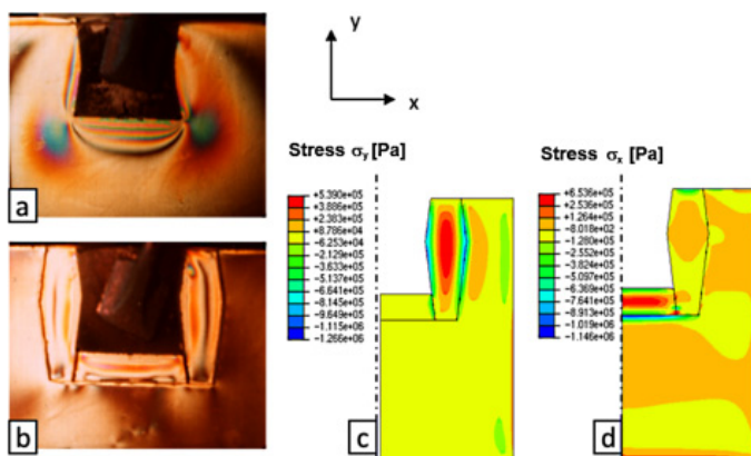
Fig. 5. Stresses visible in the zone of angular cracks after the lapse of 30 seconds since the time instant of filling the shaped groove with cast iron; a – the original design; elasto-optic image, b – the design after modifications; elasto-optic image, c, d – the design after modifications; numerical calculations
