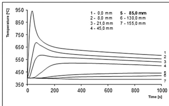
Fig. 2. Temperature changes in the cross-section of carbon block at different distances from the surface of the shaped groove.
