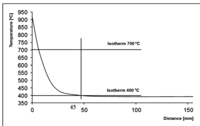
Fig. 3. Temperature changes in the cross-section of a side wall of the block during thermal shock
