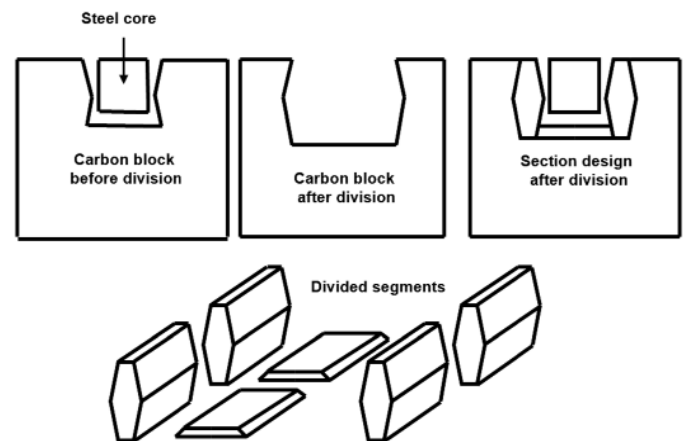
Fig. 4. A way to divide the structure of a carbon block
