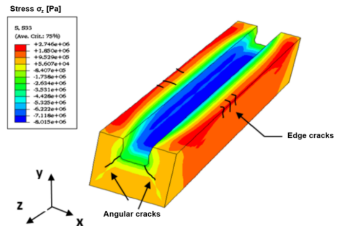
Fig. 1. Stress field \sigma_z that occurs in carbon block after the lapse of 380 seconds since the time instant of filling the shaped groove with cast iron.
