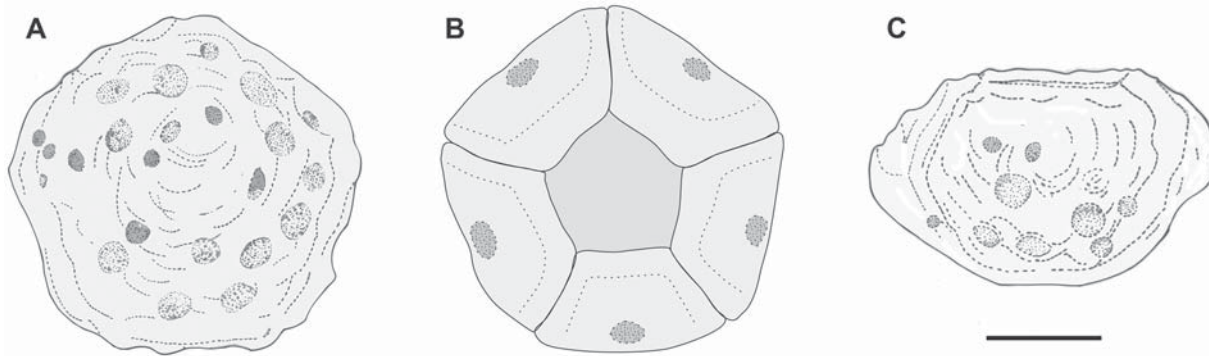
Text-fig. 6. Ink-drawing sketches of the Sievertsella cf. polonica (Radwańska): calyx (PBR-01-80) from the Miocene of the Pirabas Formation. A – Dorsal view; B – Ventral view; C – Lateral view of calyx centrodorsal plate. Scale bar = 1 mm
