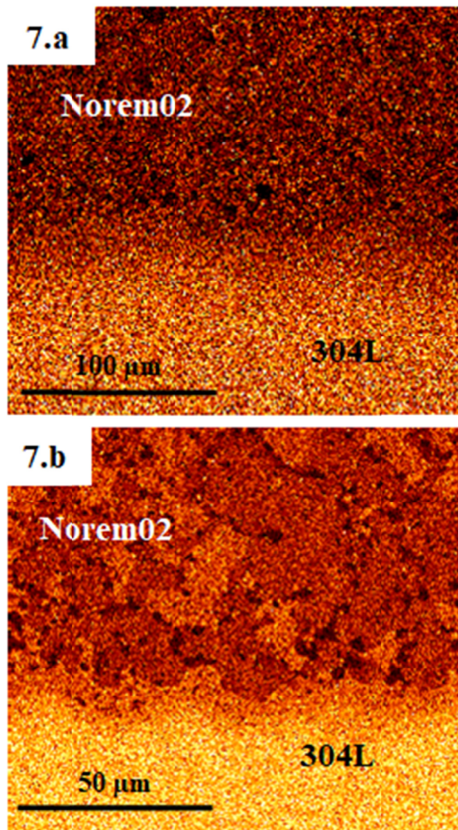
Fig. 7. SEM nickel mappings of Norem02/304L interfaces: (a) HIPed powder 1 and (b) HIPed powder 2
