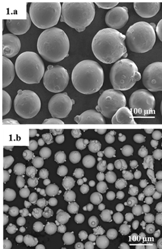
Fig. 1. SEM observations of (a) powder 1 and (b) powder 2
