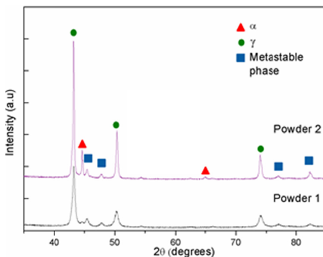
Fig. 2. XRD patterns of Norem02 powders before sintering
