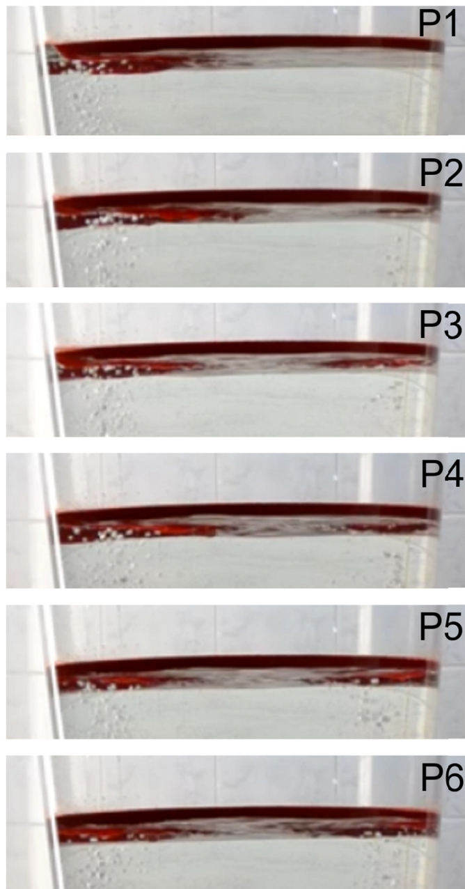
Fig. 6. The influence of the flow rate of gas and configuration of purging plugs work on the behavior of slag surface – side view
