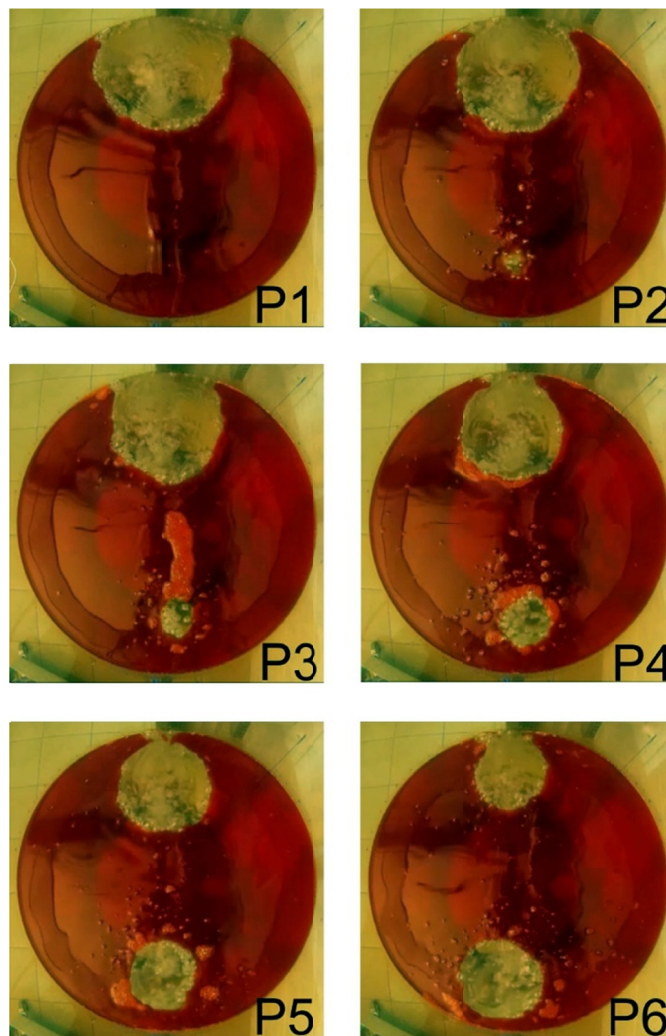
Fig. 3. The influence of flow rate of gas and configuration of purging plugs work on the size of slag eye – upper view
