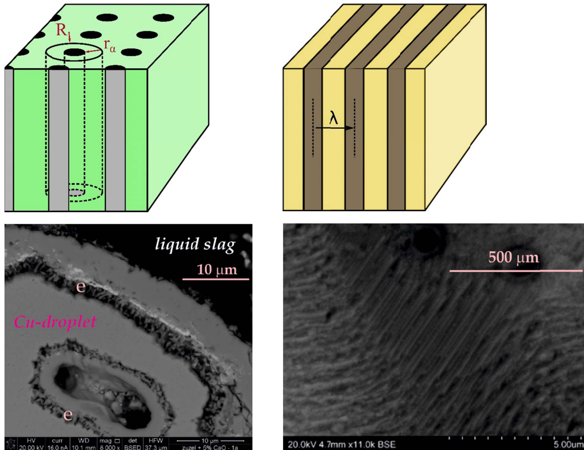
Fig. 3. Spacing in the regular structure, a) rod-like eutectic, b) lamellar eutectic, and its confirmation in the real morphology (industry condition), c) rod-like Cu-Cu 2 O – eutectic (e – area) located at the envelopes of the coagulated Cu – droplets, d) lamellar Cu-Cu 2 O – eutectic structure
