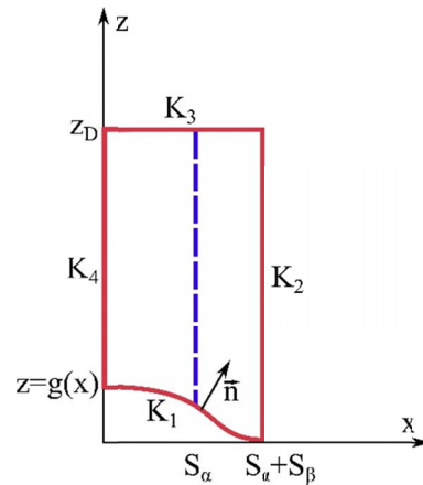
Fig. 1a. Contours applied to Eq. (5a)
