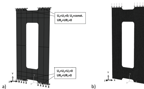
Fig. 2. Discrete model of a composite plate a) boundary conditions, b) discretization of the geometric model
